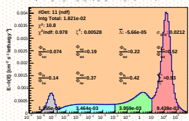
Spectrum_LCO_Event_41_Steps_16_BinSeed_154(VWC 36%)
