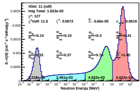
Spectrum_LCO_Event_41_Steps_6_BinSeed_154(VWC 36%)
