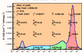
Spectrum_LCO_Event_41_Steps_18_BinSeed_154(VWC 36%)
