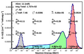
Spectrum_LCO_Event_41_Steps_7_BinSeed_154(VWC 36%)
