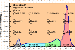
Spectrum_LCO_Event_41_Steps_20_BinSeed_154(VWC 36%)
