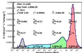
Spectrum_LCO_Event_41_Steps_14_BinSeed_154(VWC 36%)
