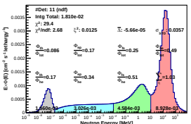
Spectrum_LCO_Event_41_Steps_12_BinSeed_154(VWC 36%)
