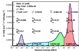
Spectrum_LCO_Event_41_Steps_9_BinSeed_154(VWC 36%)
