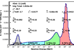
Spectrum_LCO_Event_41_Steps_10_BinSeed_154(VWC 36%)
