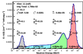
Spectrum_LCO_Event_41_Steps_8_BinSeed_154(VWC 36%)
