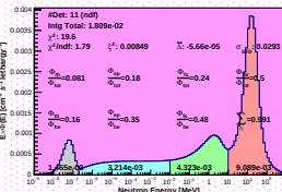
Spectrum_LCO_Event_41_Steps_15_BinSeed_154(VWC 36%)
