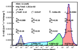
Spectrum_LCO_Event_41_Steps_11_BinSeed_154(VWC 36%)
