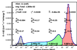
Spectrum_LCO_Event_41_Steps_13_BinSeed_154(VWC 36%)
