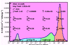
Spectrum_LCO_Event_41_Steps_17_BinSeed_154(VWC 36%)
