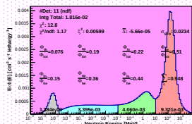
Spectrum_LCO_Event_41_Steps_19_BinSeed_154(VWC 36%)
