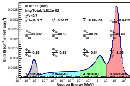
Spectrum_LCO_Event_41_Steps_10_BinSeed_155(WVC 38%)
