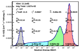
Spectrum_LCO_Event_41_Steps_6_BinSeed_155(WVC 38%)
