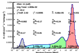
Spectrum_LCO_Event_41_Steps_14_BinSeed_155(WVC 38%)
