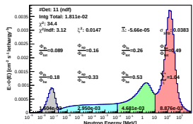
Spectrum_LCO_Event_41_Steps_11_BinSeed_155(WVC 38%)
