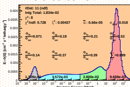
Spectrum_LCO_Event_41_Steps_20_BinSeed_155(WVC 38%)
