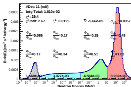
Spectrum_LCO_Event_41_Steps_12_BinSeed_155(WVC 38%)
