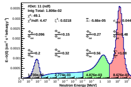
Spectrum_LCO_Event_41_Steps_9_BinSeed_155(WVC 38%)
