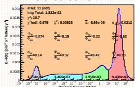
Spectrum_LCO_Event_41_Steps_16_BinSeed_155(WVC 38%)
