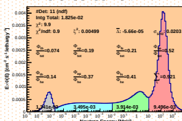
Spectrum_LCO_Event_41_Steps_17_BinSeed_155(WVC 38%)
