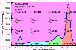
Spectrum_LCO_Event_41_Steps_15_BinSeed_155(WVC 38%)
