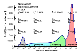
Spectrum_LCO_Event_41_Steps_13_BinSeed_155(WVC 38%)
