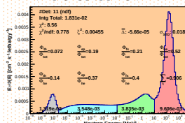
Spectrum_LCO_Event_41_Steps_19_BinSeed_155(WVC 38%)
