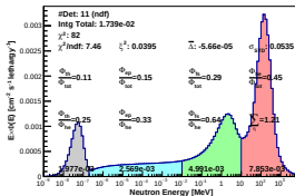
Spectrum_LCO_Event_41_Steps_7_BinSeed_155(WVC 38%)
