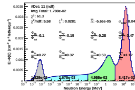
Spectrum_LCO_Event_41_Steps_8_BinSeed_155(WVC 38%)
