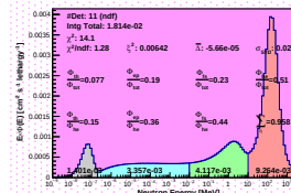
Spectrum_LCO_Event_41_Steps_18_BinSeed_155(WVC 38%)
