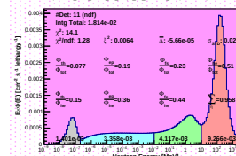
Spectrum_LCO_Event_41_Steps_18_BinSead_156(WVC 40%)
