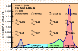
Spectrum_LCO_Event_41_Steps_17_BinSead_156(WVC 40%)
