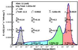
Spectrum_LCO_Event_41_Steps_6_BinSead_156(WVC 40%)
