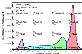
Spectrum_LCO_Event_41_Steps_12_BinSead_156(WVC 40%)
