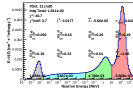
Spectrum_LCO_Event_41_Steps_10_BinSead_156(WVC 40%)
