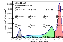
Spectrum_LCO_Event_41_Steps_9_BinSead_156(WVC 40%)
