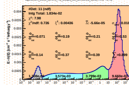
Spectrum_LCO_Event_41_Steps_20_BinSead_156(WVC 40%)
