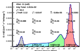
Spectrum_LCO_Event_41_Steps_11_BinSead_156(WVC 40%)
