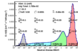
Spectrum_LCO_Event_41_Steps_8_BinSead_156(WVC 40%)
