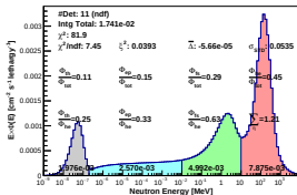
Spectrum_LCO_Event_41_Steps_7_BinSead_156(WVC 40%)
