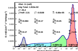
Spectrum_LCO_Event_41_Steps_13_BinSead_156(WVC 40%)
