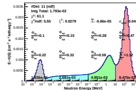
Spectrum_LCO_Event_41_Steps_8_BinSead_160(WVC 48%)
