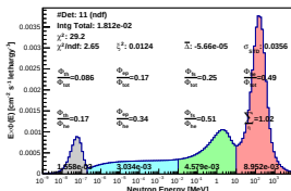
Spectrum_LCO_Event_41_Steps_12_BinSead_160(WVC 48%)
