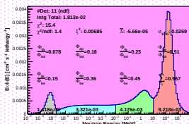
Spectrum_LCO_Event_41_Steps_17_BinSead_160(WVC 48%)
