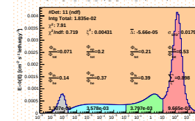
Spectrum_LCO_Event_41_Steps_20_BinSead_160(WVC 48%)
