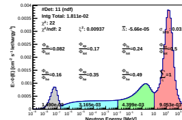
Spectrum_LCO_Event_41_Steps_14_BinSead_160(WVC 48%)
