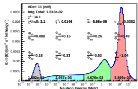
Spectrum_LCO_Event_41_Steps_11_BinSead_160(WVC 48%)
