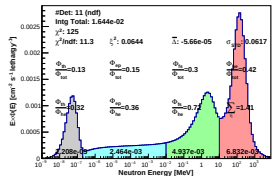
Spectrum_LCO_Event_41_Steps_6_BinSead_160(WVC 48%)
