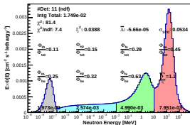
Spectrum_LCO_Event_41_Steps_7_BinSead_160(WVC 48%)
