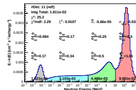
Spectrum_LCO_Event_41_Steps_13_BinSead_160(WVC 48%)
