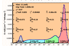
Spectrum_LCO_Event_41_Steps_18_BinSead_160(WVC 48%)
