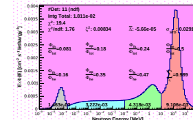
Spectrum_LCO_Event_41_Steps_15_BinSead_160(WVC 48%)
