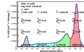
Spectrum_LCO_Event_41_Steps_10_BinSead_160(WVC 48%)
