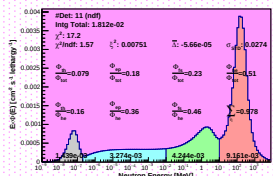
Spectrum_LCO_Event_41_Steps_16_BinSead_160(WVC 48%)
