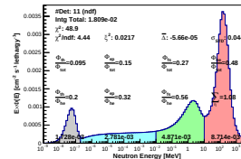
Spectrum_LCO_Event_41_Steps_9_BinSead_160(WVC 48%)
