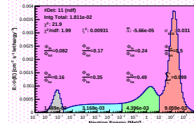
Spectrum_LCO_Event_14_Steps_14_BinSeed_162(WVC 52%)
