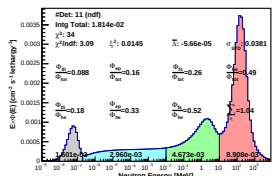
Spectrum_LCO_Event_11_Steps_11_BinSeed_162(WVC 52%)
