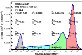
Spectrum_LCO_Event_7_Steps_7_BinSeed_162(WVC 52%)
