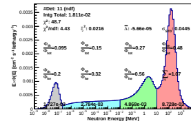
Spectrum_LCO_Event_9_Steps_9_BinSeed_162(WVC 52%)
