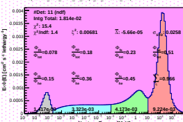
Spectrum_LCO_Event_17_Steps_17_BinSeed_162(WVC 52%)
