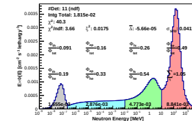
Spectrum_LCO_Event_10_Steps_10_BinSeed_162(WVC 52%)
