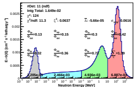
Spectrum_LCO_Event_6_Steps_6_BinSeed_162(WVC 52%)
