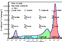
Spectrum_LCO_Event_12_Steps_12_BinSeed_162(WVC 52%)
