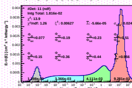
Spectrum_LCO_Event_18_Steps_18_BinSeed_162(WVC 52%)
