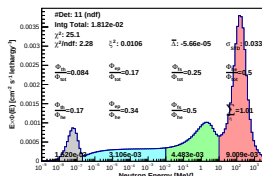
Spectrum_LCO_Event_13_Steps_13_BinSeed_162(WVC 52%)
