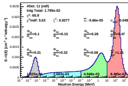
Spectrum_LCO_Event_8_Steps_8_BinSeed_162(WVC 52%)
