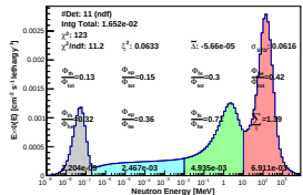
Spectrum_LCO_Event_41_Steps_6_BinSeed_163(WVC 54%)
