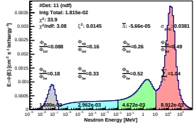
Spectrum_LCO_Event_41_Steps_11_BinSeed_163(WVC 54%)
