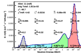
Spectrum_LCO_Event_41_Steps_9_BinSeed_163(WVC 54%)
