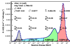
Spectrum_LCO_Event_41_Steps_8_BinSeed_163(WVC 54%)
