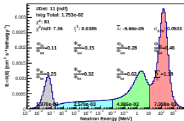
Spectrum_LCO_Event_41_Steps_7_BinSeed_163(WVC 54%)
