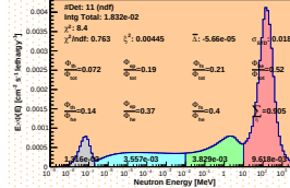
Spectrum_LCO_Event_41_Steps_19_BinSeed_163(WVC 54%)
