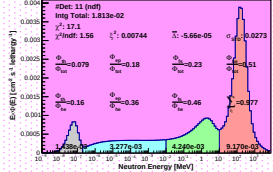
Spectrum_LCO_Event_41_Steps_16_BinSeed_163(WVC 54%)
