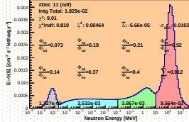
Spectrum_LCO_Event_41_Steps_18_BinSeed_163(WVC 54%)
