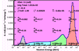
Spectrum_LCO_Event_41_Steps_14_BinSeed_163(WVC 54%)
