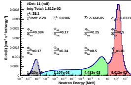
Spectrum_LCO_Event_41_Steps_13_BinSeed_163(WVC 54%)
