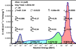
Spectrum_LCO_Event_41_Steps_12_BinSeed_163(WVC 54%)
