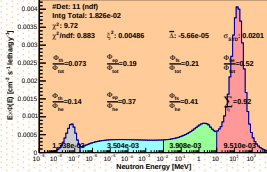
Spectrum_LCO_Event_41_Steps_17_BinSeed_163(WVC 54%)
