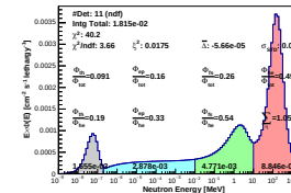
Spectrum_LCO_Event_41_Steps_10_BinSeed_163(WVC 54%)
