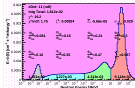
Spectrum_LCO_Event_41_Steps_15_BinSeed_164(WVC 56%)
