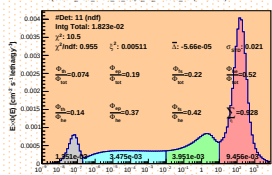
Spectrum_LCO_Event_41_Steps_16_BinSeed_164(WVC 56%)
