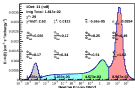
Spectrum_LCO_Event_41_Steps_12_BinSeed_164(WVC 56%)
