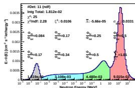
Spectrum_LCO_Event_41_Steps_13_BinSeed_164(WVC 56%)
