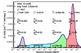
Spectrum_LCO_Event_41_Steps_10_BinSeed_164(WVC 56%)
