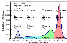
Spectrum_LCO_Event_41_Steps_11_BinSeed_164(WVC 56%)
