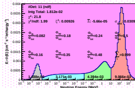
Spectrum_LCO_Event_41_Steps_14_BinSeed_164(WVC 56%)
