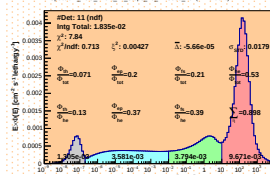
Spectrum_LCO_Event_41_Steps_20_BinSeed_164(WVC 56%)
