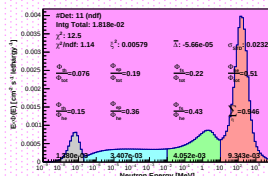
Spectrum_LCO_Event_41_Steps_19_BinSeed_164(WVC 56%)
