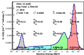
Spectrum_LCO_Event_41_Steps_7_BinSeed_164(WVC 56%)
