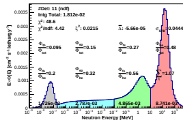
Spectrum_LCO_Event_41_Steps_9_BinSeed_164(WVC 56%)
