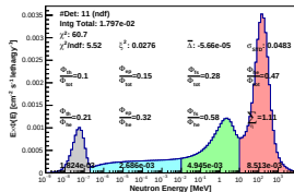
Spectrum_LCO_Event_41_Steps_8_BinSeed_164(WVC 56%)
