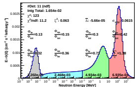
Spectrum_LCO_Event_41_Steps_6_BinSeed_164(WVC 56%)
