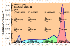
Spectrum_LCO_Event_41_Steps_18_BinSeed_164(WVC 56%)
