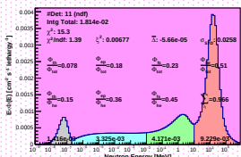
Spectrum_LCO_Event_41_Steps_17_BinSeed_164(WVC 56%)
