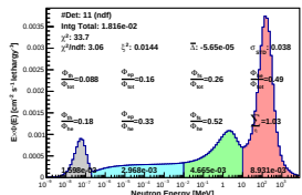
Spectrum_LCO_Event_41_Steps_11_BinSeed_168(WVC 64%)
