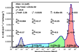
Spectrum_LCO_Event_41_Steps_13_BinSeed_168(WVC 64%)
