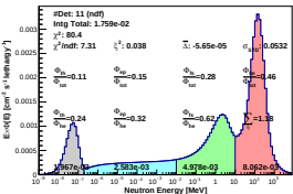
Spectrum_LCO_Event_41_Steps_7_BinSeed_168(WVC 64%)
