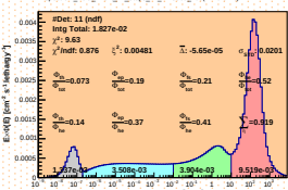
Spectrum_LCO_Event_41_Steps_17_BinSeed_168(WVC 64%)
