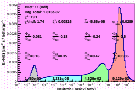
Spectrum_LCO_Event_41_Steps_15_BinSeed_168(WVC 64%)
