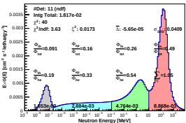
Spectrum_LCO_Event_41_Steps_10_BinSeed_168(WVC 64%)
