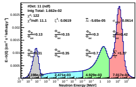
Spectrum_LCO_Event_41_Steps_6_BinSeed_168(WVC 64%)
