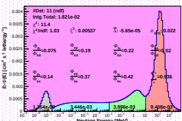
Spectrum_LCO_Event_41_Steps_20_BinSeed_168(WVC 64%)
