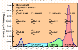
Spectrum_LCO_Event_41_Steps_16_BinSeed_168(WVC 64%)
