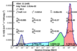
Spectrum_LCO_Event_41_Steps_9_BinSeed_168(WVC 64%)
