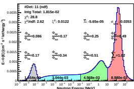
Spectrum_LCO_Event_41_Steps_12_BinSeed_168(WVC 64%)
