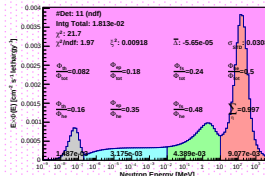
Spectrum_LCO_Event_41_Steps_14_BinSeed_168(WVC 64%)
