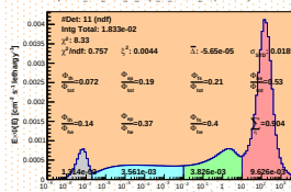
Spectrum_LCO_Event_41_Steps_19_BinSeed_168(WVC 64%)
