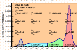
Spectrum_LCO_Event_41_Steps_18_BinSeed_168(WVC 64%)
