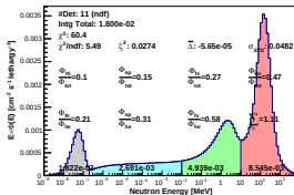
Spectrum_LCO_Event_41_Steps_8_BinSeed_168(WVC 64%)
