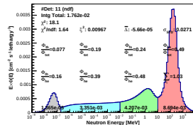
Spectrum_LCO_Event_41_Staps_9_BinSeed_17(WVC 3.2%)
