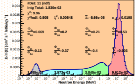
Spectrum_LCO_Event_41_Staps_16_BinSeed_17(WVC 3.2%)
