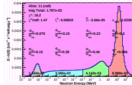
Spectrum_LCO_Event_41_Staps_10_BinSeed_17(WVC 3.2%)
