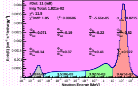
Spectrum_LCO_Event_41_Staps_14_BinSeed_17(WVC 3.2%)
