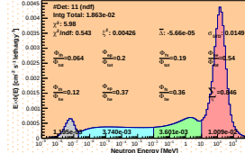
Spectrum_LCO_Event_41_Staps_20_BinSeed_17(WVC 3.2%)
