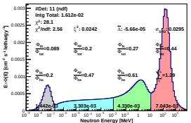
Spectrum_LCO_Event_41_Staps_7_BinSeed_17(WVC 3.2%)
