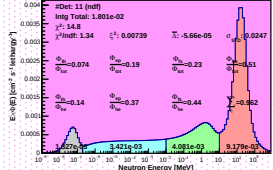
Spectrum_LCO_Event_41_Staps_11_BinSeed_17(WVC 3.2%)
