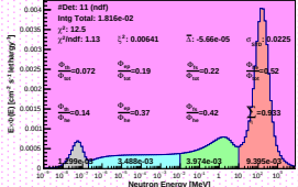
Spectrum_LCO_Event_41_Staps_13_BinSeed_17(WVC 3.2%)
