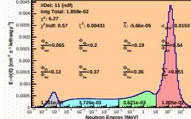
Spectrum_LCO_Event_41_Staps_19_BinSeed_17(WVC 3.2%)
