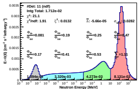
Spectrum_LCO_Event_41_Staps_3_BinSeed_17(WVC 3.2%)
