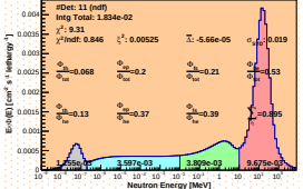
Spectrum_LCO_Event_41_Staps_17_BinSeed_17(WVC 3.2%)
