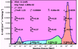
Spectrum_LCO_Event_41_Staps_12_BinSeed_17(WVC 3.2%)
