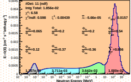
Spectrum_LCO_Event_41_Staps_18_BinSeed_17(WVC 3.2%)
