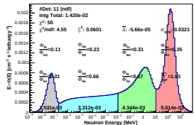
Spectrum_LCO_Event_41_Staps_8_BinSeed_17(WVC 3.2%)
