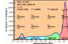
Spectrum_LCO_Event_41_Staps_15_BinSead_18(WVC 3.4%)
