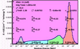
Spectrum_LCO_Event_41_Staps_11_BinSead_18(WVC 3.4%)
