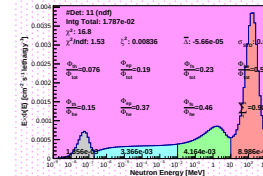
Spectrum_LCO_Event_41_Staps_10_BinSead_18(WVC 3.4%)
