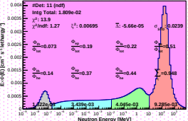
Spectrum_LCO_Event_41_Staps_12_BinSead_18(WVC 3.4%)
