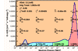
Spectrum_LCO_Event_41_Staps_20_BinSead_18(WVC 3.4%)
