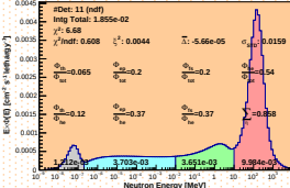
Spectrum_LCO_Event_41_Staps_18_BinSead_18(WVC 3.4%)
