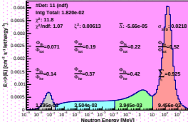
Spectrum_LCO_Event_41_Staps_14_BinSead_18(WVC 3.4%)
