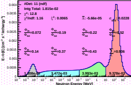
Spectrum_LCO_Event_41_Staps_13_BinSead_18(WVC 3.4%)
