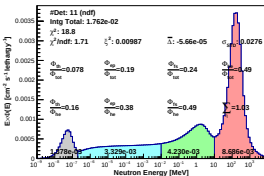
Spectrum_LCO_Event_41_Staps_9_BinSead_18(WVC 3.4%)
