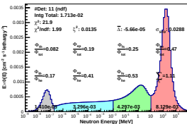
Spectrum_LCO_Event_41_Staps_8_BinSead_18(WVC 3.4%)
