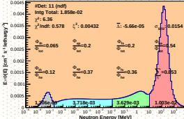
Spectrum_LCO_Event_41_Staps_19_BinSead_18(WVC 3.4%)
