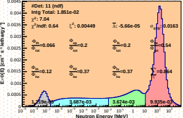
Spectrum_LCO_Event_41_Staps_17_BinSead_18(WVC 3.4%)
