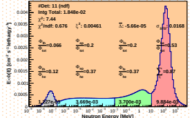
Spectrum_LCO_Event_41_Staps_16_BinSead_18(WVC 3.4%)
