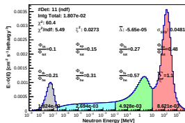
Spectrum_LCO_Event_8_BinSeed_133(WVC 94%)
