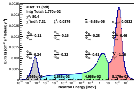
Spectrum_LCO_Event_7_BinSeed_133(WVC 94%)
