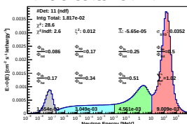
Spectrum_LCO_Event_12_BinSeed_133(WVC 94%)
