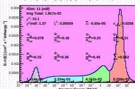
Spectrum_LCO_Event_17_BinSeed_133(WVC 94%)
