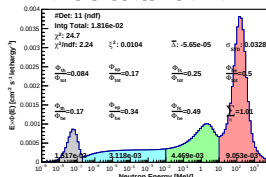
Spectrum_LCO_Event_13_BinSeed_133(WVC 94%)
