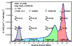
Spectrum_LCO_Event_6_BinSeed_133(WVC 94%)
