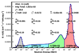
Spectrum_LCO_Event_10_BinSeed_133(WVC 94%)
