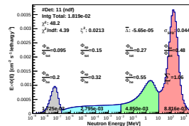
Spectrum_LCO_Event_9_BinSeed_133(WVC 94%)
