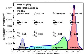
Spectrum_LCO_Event_11_BinSeed_133(WVC 94%)
