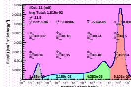
Spectrum_LCO_Event_14_BinSeed_133(WVC 94%)
