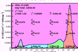
Spectrum_LCO_Event_20_BinSeed_133(WVC 94%)
