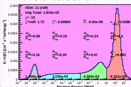
Spectrum_LCO_Event_15_BinSeed_133(WVC 94%)
