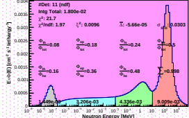
Spectrum_LCO_Event_41_Staps_11_BinSeed_33(VWC 6.4%)
