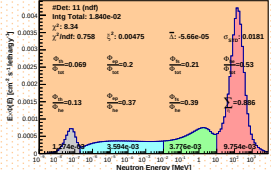
Spectrum_LCO_Event_41_Staps_17_BinSeed_33(VWC 6.4%)
