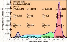
Spectrum_LCO_Event_41_Staps_19_BinSeed_33(VWC 6.4%)
