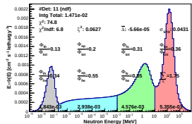
Spectrum_LCO_Event_41_Staps_6_BinSeed_33(VWC 6.4%)
