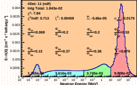
Spectrum_LCO_Event_41_Staps_18_BinSeed_33(VWC 6.4%)
