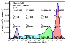
Spectrum_LCO_Event_41_Staps_7_BinSeed_33(VWC 6.4%)
