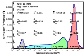
Spectrum_LCO_Event_41_Staps_10_BinSeed_33(VWC 6.4%)
