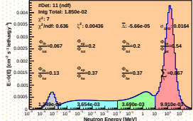
Spectrum_LCO_Event_41_Staps_20_BinSeed_33(VWC 6.4%)
