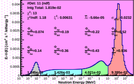
Spectrum_LCO_Event_41_Staps_16_BinSeed_33(VWC 6.4%)
