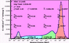
Spectrum_LCO_Event_41_Staps_14_BinSeed_33(VWC 6.4%)
