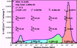
Spectrum_LCO_Event_41_Staps_13_BinSeed_33(VWC 6.4%)
