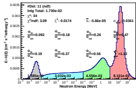
Spectrum_LCO_Event_41_Staps_8_BinSeed_33(VWC 6.4%)
