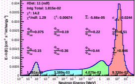
Spectrum_LCO_Event_41_Staps_15_BinSeed_33(VWC 6.4%)
