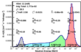
Spectrum_LCO_Event_41_Staps_9_BinSeed_33(VWC 6.4%)
