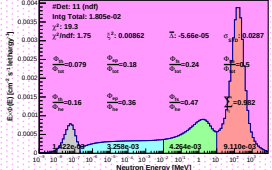
Spectrum_LCO_Event_41_Staps_12_BinSeed_33(VWC 6.4%)
