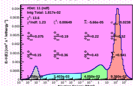
Spectrum_LCO_Event_41_Steps_16_BinSeed_37(VWC 7.2%)
