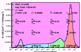
Spectrum_LCO_Event_41_Steps_15_BinSeed_37(VWC 7.2%)
