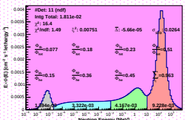
Spectrum_LCO_Event_41_Steps_14_BinSeed_37(VWC 7.2%)
