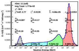
Spectrum_LCO_Event_41_Steps_9_BinSeed_37(VWC 7.2%)
