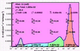
Spectrum_LCO_Event_41_Steps_12_BinSeed_37(VWC 7.2%)
