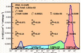
Spectrum_LCO_Event_41_Steps_20_BinSeed_37(VWC 7.2%)
