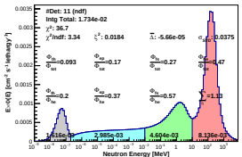
Spectrum_LCO_Event_41_Steps_8_BinSeed_37(VWC 7.2%)
