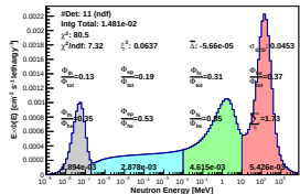
Spectrum_LCO_Event_41_Steps_6_BinSeed_37(VWC 7.2%)
