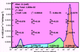
Spectrum_LCO_Event_41_Steps_13_BinSeed_37(VWC 7.2%)
