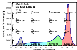
Spectrum_LCO_Event_41_Steps_11_BinSeed_37(VWC 7.2%)
