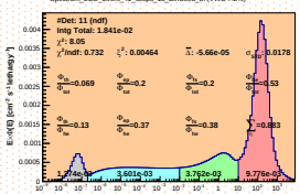
Spectrum_LCO_Event_41_Steps_18_BinSeed_37(VWC 7.2%)
