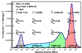
Spectrum_LCO_Event_41_Steps_7_BinSeed_37(VWC 7.2%)
