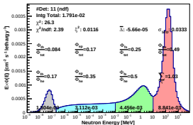
Spectrum_LCO_Event_41_Steps_10_BinSeed_37(VWC 7.2%)
