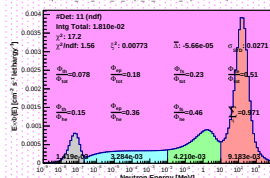
Spectrum_LCO_Event_41_Steps_15_BinSd_57(WVC 11.2%)
