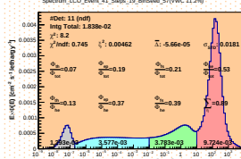
Spectrum_LCO_Event_41_Steps_19_BinSd_57(WVC 11.2%)
