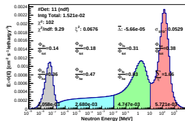
Spectrum_LCO_Event_41_Steps_6_BinSd_57(WVC 11.2%)
