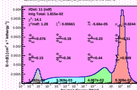
Spectrum_LCO_Event_41_Steps_17_BinSd_57(WVC 11.2%)
