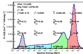
Spectrum_LCO_Event_41_Steps_7_BinSd_57(WVC 11.2%)
