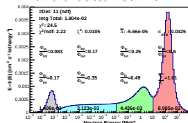
Spectrum_LCO_Event_41_Steps_12_BinSd_57(WVC 11.2%)
