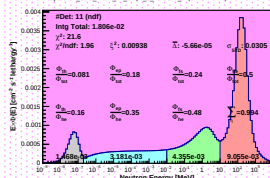
Spectrum_LCO_Event_41_Steps_13_BinSd_57(WVC 11.2%)
