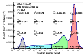
Spectrum_LCO_Event_41_Steps_9_BinSd_57(WVC 11.2%)
