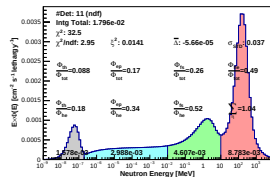
Spectrum_LCO_Event_41_Steps_10_BinSd_57(WVC 11.2%)
