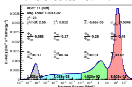
Spectrum_LCO_Event_41_Steps_11_BinSd_57(WVC 11.2%)
