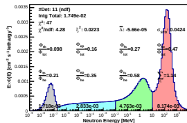
Spectrum_LCO_Event_41_Steps_8_BinSd_57(WVC 11.2%)
