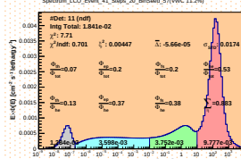
Spectrum_LCO_Event_41_Steps_20_BinSd_57(WVC 11.2%)
