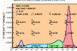
Spectrum_LCO_Event_41_Steps_18_BinSd_57(WVC 11.2%)
