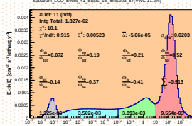
Spectrum_LCO_Event_41_Steps_16_BinSd_57(WVC 11.2%)
