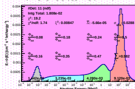
Spectrum_LCO_Event_41_Steps_14_BinSd_57(WVC 11.2%)
