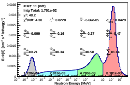
Spectrum_LCO_Event_41_Steps_8_BinSd_60(VWC 11.8%)
