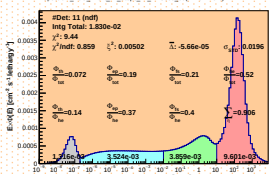
Spectrum_LCO_Event_41_Steps_17_BinSd_60(VWC 11.8%)
