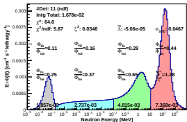
Spectrum_LCO_Event_41_Steps_7_BinSd_60(VWC 11.8%)
