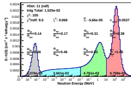
Spectrum_LCO_Event_41_Steps_6_BinSd_60(VWC 11.8%)
