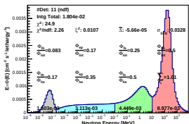
Spectrum_LCO_Event_41_Steps_12_BinSd_60(VWC 11.8%)
