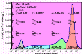
Spectrum_LCO_Event_41_Steps_14_BinSd_60(VWC 11.8%)
