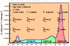
Spectrum_LCO_Event_41_Steps_18_BinSd_60(VWC 11.8%)
