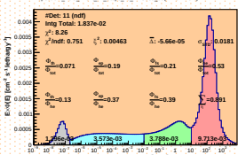
Spectrum_LCO_Event_41_Steps_19_BinSd_60(VWC 11.8%)
