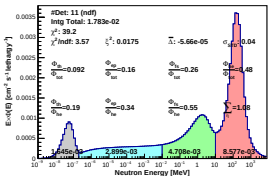
Spectrum_LCO_Event_41_Steps_9_BinSd_60(VWC 11.8%)
