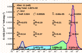
Spectrum_LCO_Event_41_Steps_16_BinSd_60(VWC 11.8%)
