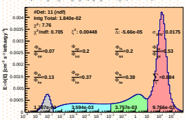
Spectrum_LCO_Event_41_Steps_20_BinSd_60(VWC 11.8%)
