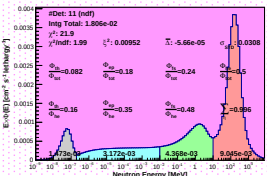
Spectrum_LCO_Event_41_Steps_13_BinSd_60(VWC 11.8%)
