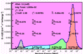
Spectrum_LCO_Event_41_Steps_15_BinSd_60(VWC 11.8%)
