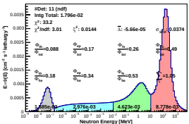
Spectrum_LCO_Event_41_Steps_10_BinSd_60(VWC 11.8%)
