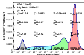
Spectrum_LCO_Event_41_Steps_11_BinSd_60(VWC 11.8%)
