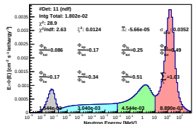
Spectrum_LCO_Event_41_Steps_11_BinSd_62(WVC 12.2%)
