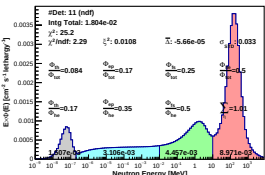
Spectrum_LCO_Event_41_Steps_12_BinSd_62(WVC 12.2%)
