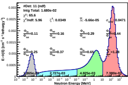
Spectrum_LCO_Event_41_Steps_7_BinSd_62(WVC 12.2%)
