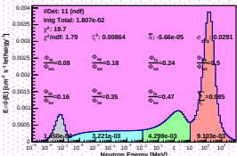
Spectrum_LCO_Event_41_Steps_14_BinSd_62(WVC 12.2%)
