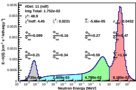
Spectrum_LCO_Event_41_Steps_8_BinSd_62(WVC 12.2%)
