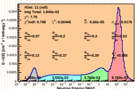
Spectrum_LCO_Event_41_Steps_20_BinSd_62(WVC 12.2%)
