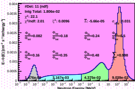
Spectrum_LCO_Event_41_Steps_13_BinSd_62(WVC 12.2%)
