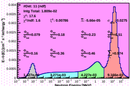
Spectrum_LCO_Event_41_Steps_15_BinSd_62(WVC 12.2%)
