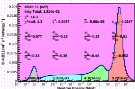
Spectrum_LCO_Event_41_Steps_17_BinSd_62(WVC 12.2%)
