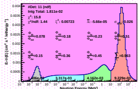
Spectrum_LCO_Event_41_Steps_16_BinSd_62(WVC 12.2%)
