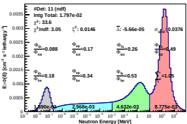
Spectrum_LCO_Event_41_Steps_10_BinSd_62(WVC 12.2%)
