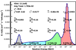
Spectrum_LCO_Event_41_Steps_9_BinSd_62(WVC 12.2%)
