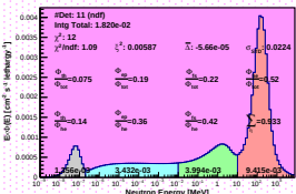
Spectrum_LCO_Event_41_Steps_19_BinSd_62(WVC 12.2%)
