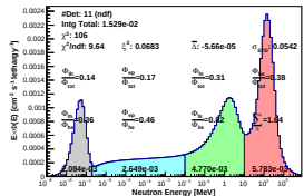
Spectrum_LCO_Event_41_Steps_6_BinSd_62(WVC 12.2%)
