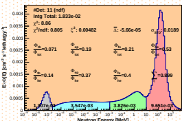
Spectrum_LCO_Event_41_Steps_18_BinSd_62(WVC 12.2%)
