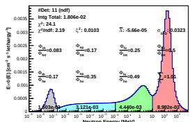
Spectrum_LCO_Event_41_Steps_13_BinSd_87(WVC 17.2%)
