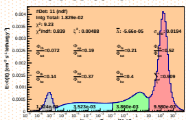
Spectrum_LCO_Event_41_Steps_18_BinSeid_97(WVC 19.2%)
