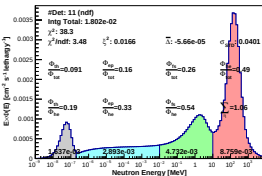
Spectrum_LCO_Event_41_Steps_10_BinSeid_97(WVC 19.2%)
