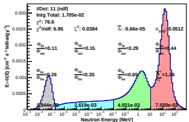
Spectrum_LCO_Event_41_Steps_7_BinSeid_97(WVC 19.2%)
