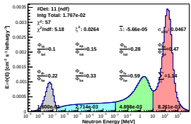
Spectrum_LCO_Event_41_Steps_8_BinSeid_97(WVC 19.2%)
