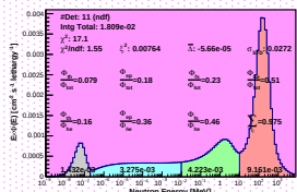
Spectrum_LCO_Event_41_Steps_16_BinSeid_97(WVC 19.2%)
