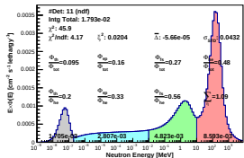
Spectrum_LCO_Event_41_Steps_9_BinSeid_97(WVC 19.2%)
