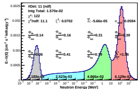
Spectrum_LCO_Event_41_Steps_6_BinSeid_97(WVC 19.2%)
