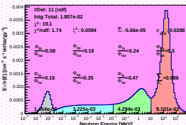
Spectrum_LCO_Event_41_Steps_15_BinSeid_97(WVC 19.2%)
