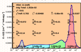
Spectrum_LCO_Event_41_Steps_19_BinSeid_97(WVC 19.2%)
