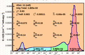
Spectrum_LCO_Event_41_Steps_17_BinSeid_97(WVC 19.2%)
