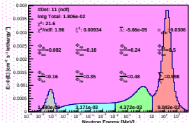
Spectrum_LCO_Event_41_Steps_14_BinSeid_97(WVC 19.2%)
