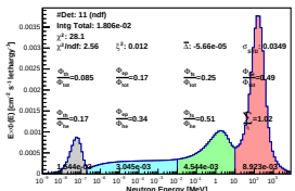
Spectrum_LCO_Event_41_Steps_12_BinSeid_97(WVC 19.2%)
