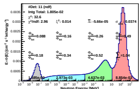
Spectrum_LCO_Event_41_Steps_11_BinSeid_97(WVC 19.2%)
