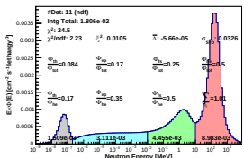
Spectrum_LCO_Event_41_Steps_13_BinSeid_97(WVC 19.2%)
