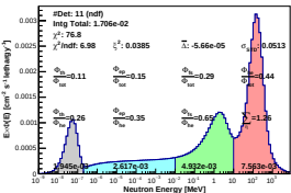
Spectrum_LCO_Event_41_Steps_7_BinSeed_98(WVC 19.4%)
