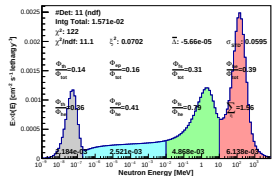
Spectrum_LCO_Event_41_Steps_6_BinSeed_98(WVC 19.4%)
