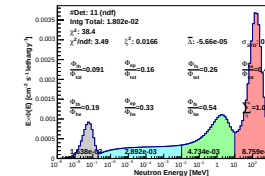
Spectrum_LCO_Event_41_Steps_10_BinSeed_98(WVC 19.4%)
