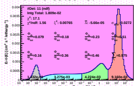
Spectrum_LCO_Event_41_Steps_16_BinSeed_98(WVC 19.4%)
