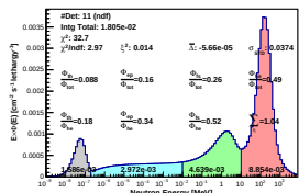
Spectrum_LCO_Event_41_Steps_11_BinSeed_98(WVC 19.4%)
