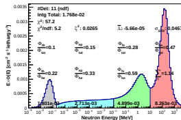
Spectrum_LCO_Event_41_Steps_8_BinSeed_98(WVC 19.4%)
