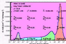
Spectrum_LCO_Event_41_Steps_14_BinSeed_98(WVC 19.4%)
