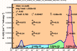
Spectrum_LCO_Event_41_Steps_19_BinSeed_98(WVC 19.4%)
