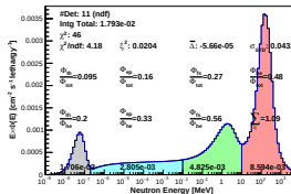
Spectrum_LCO_Event_41_Steps_9_BinSeed_98(WVC 19.4%)
