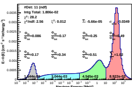
Spectrum_LCO_Event_41_Steps_12_BinSeed_98(WVC 19.4%)
