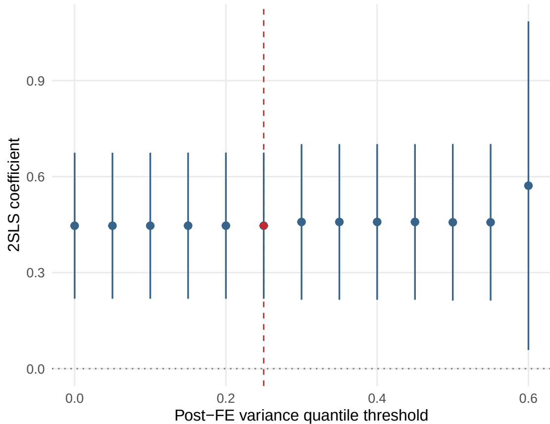
Municipality: coefficient stability
