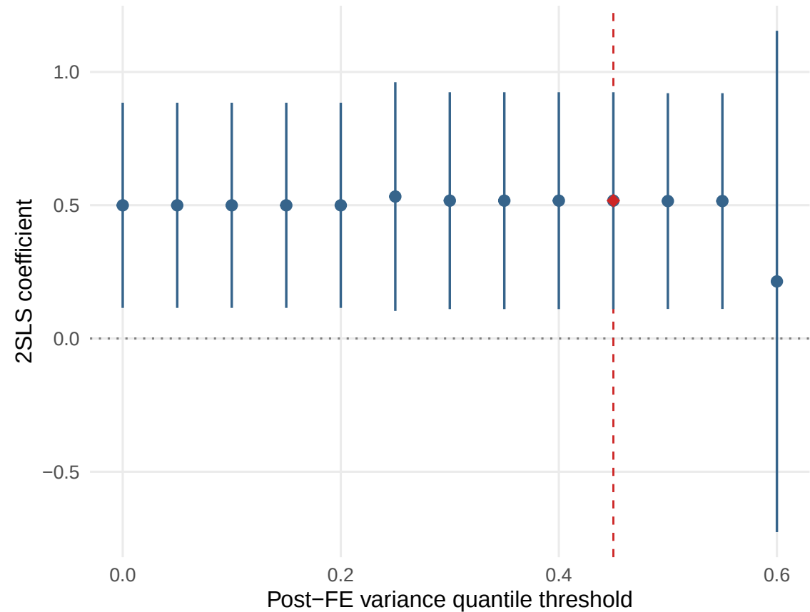
DSEI polo base: coefficient stability
