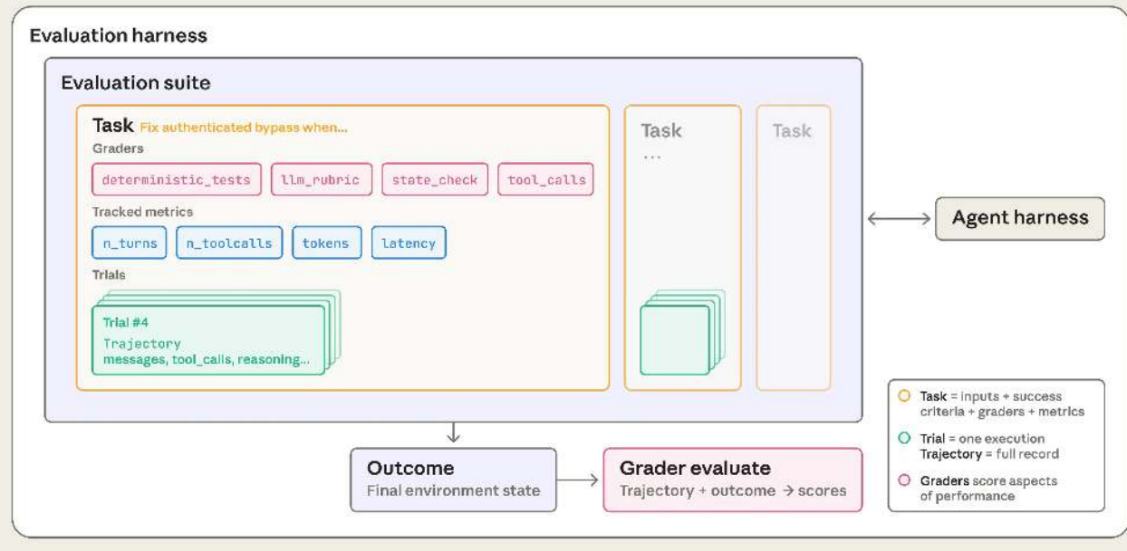
Components of evaluations for agents.
