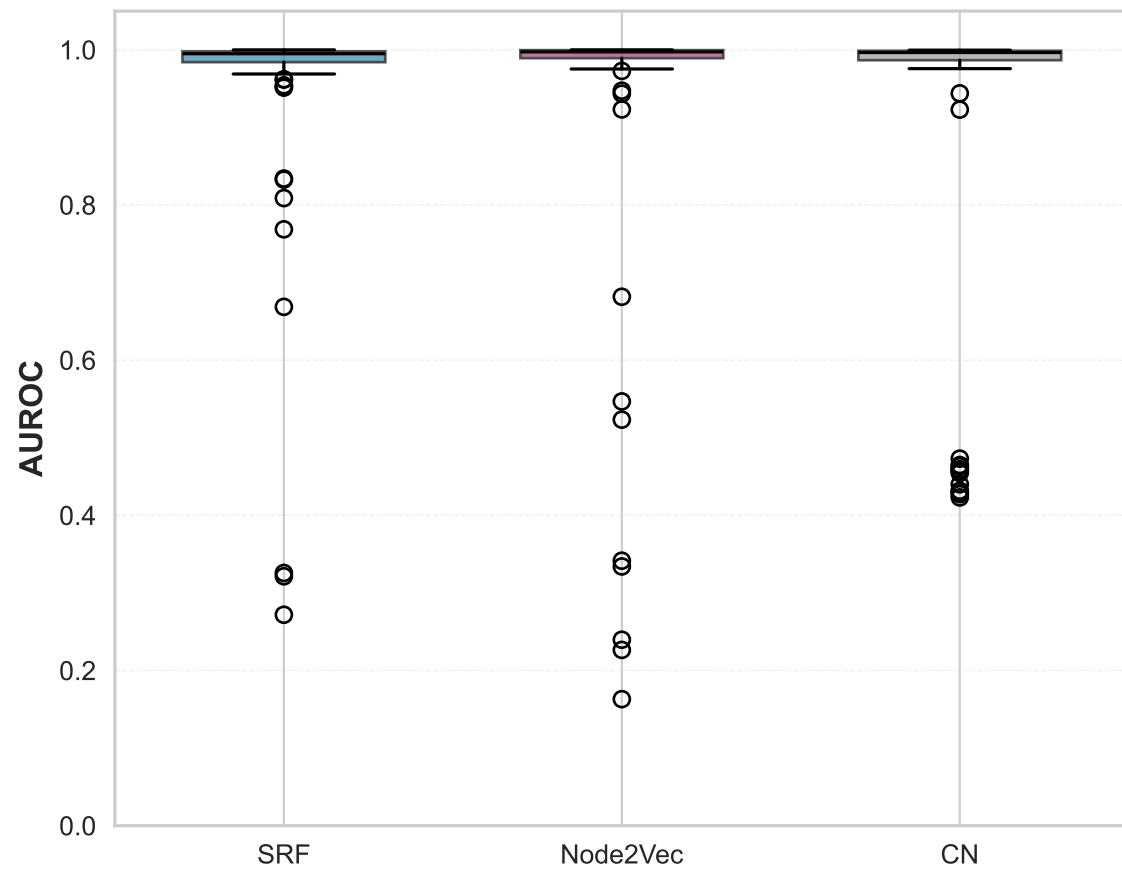
AUROC distribution
