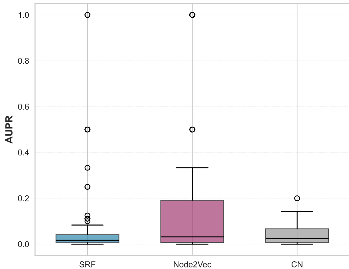
AUPR distribution
