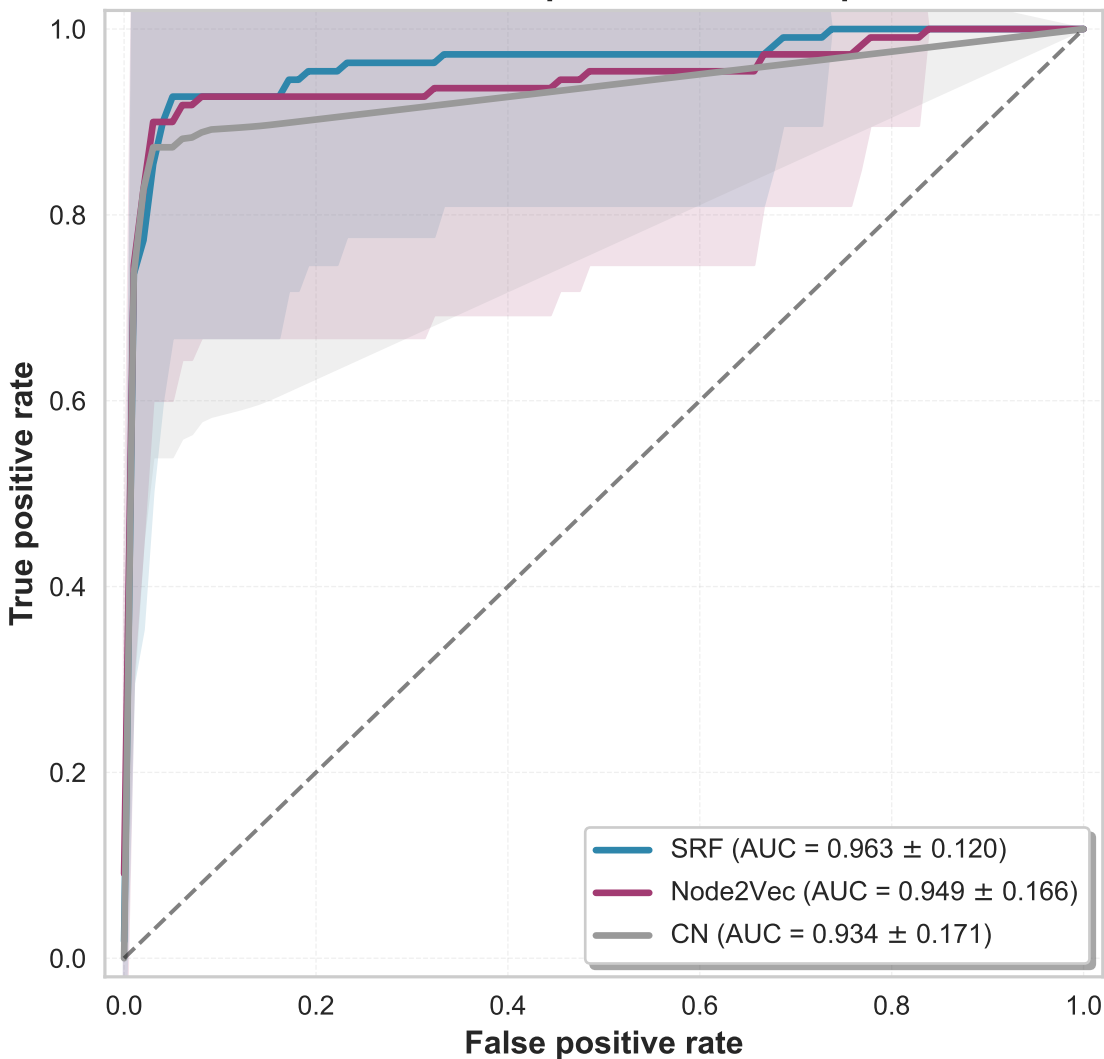
ROC curves: complex member completion
