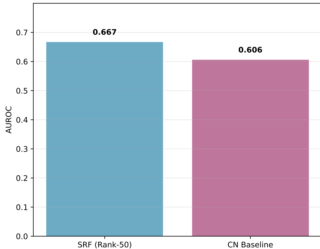
Cross-Dataset Validation: AUROC
