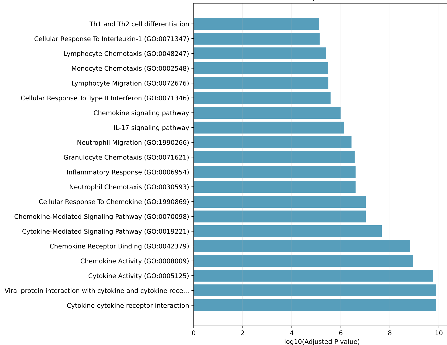
Factor 18: top enriched terms
