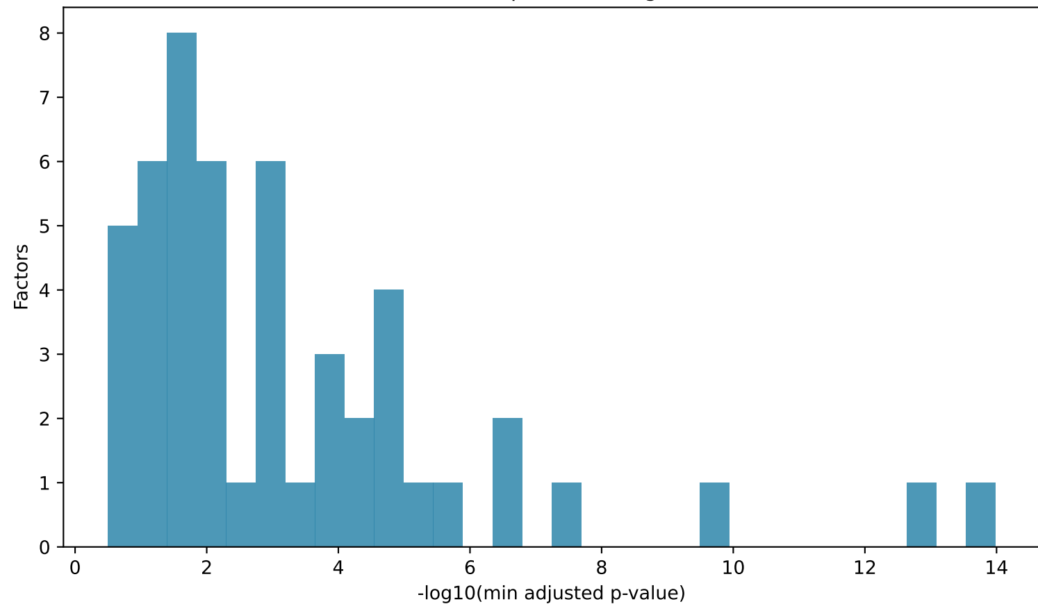
Distribution of per-factor significance
