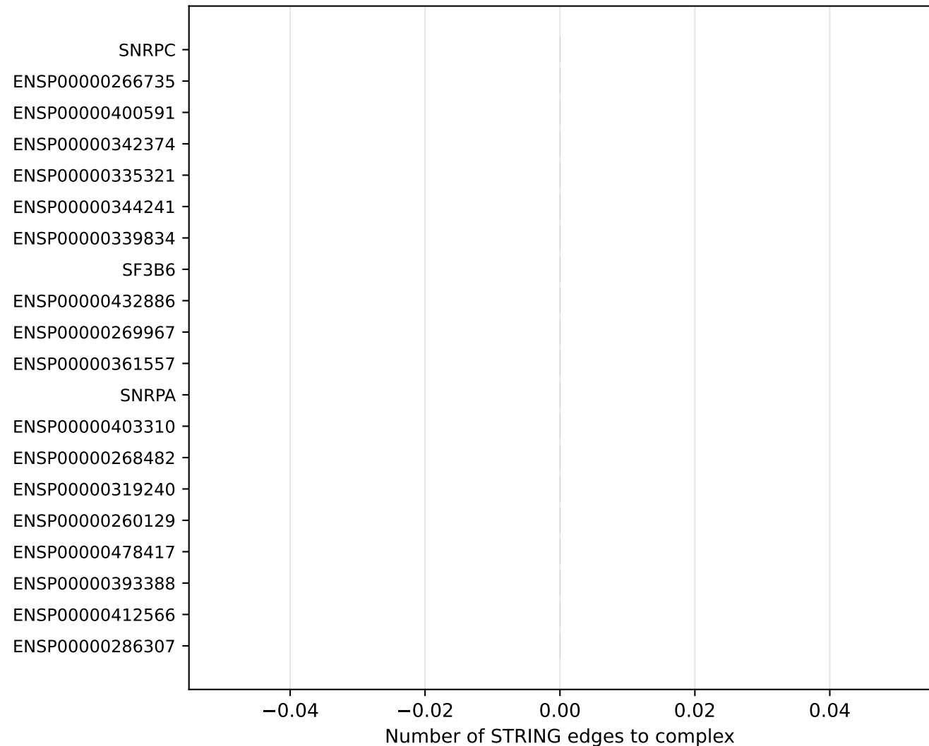
C complex spliceosome: STRING evidence
