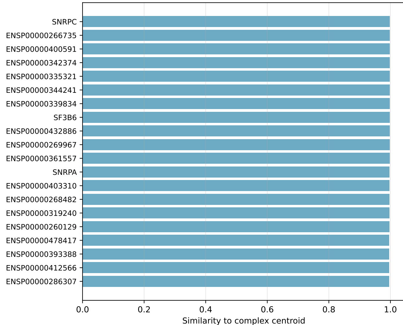
C complex spliceosome: top candidates by embedding similarity
