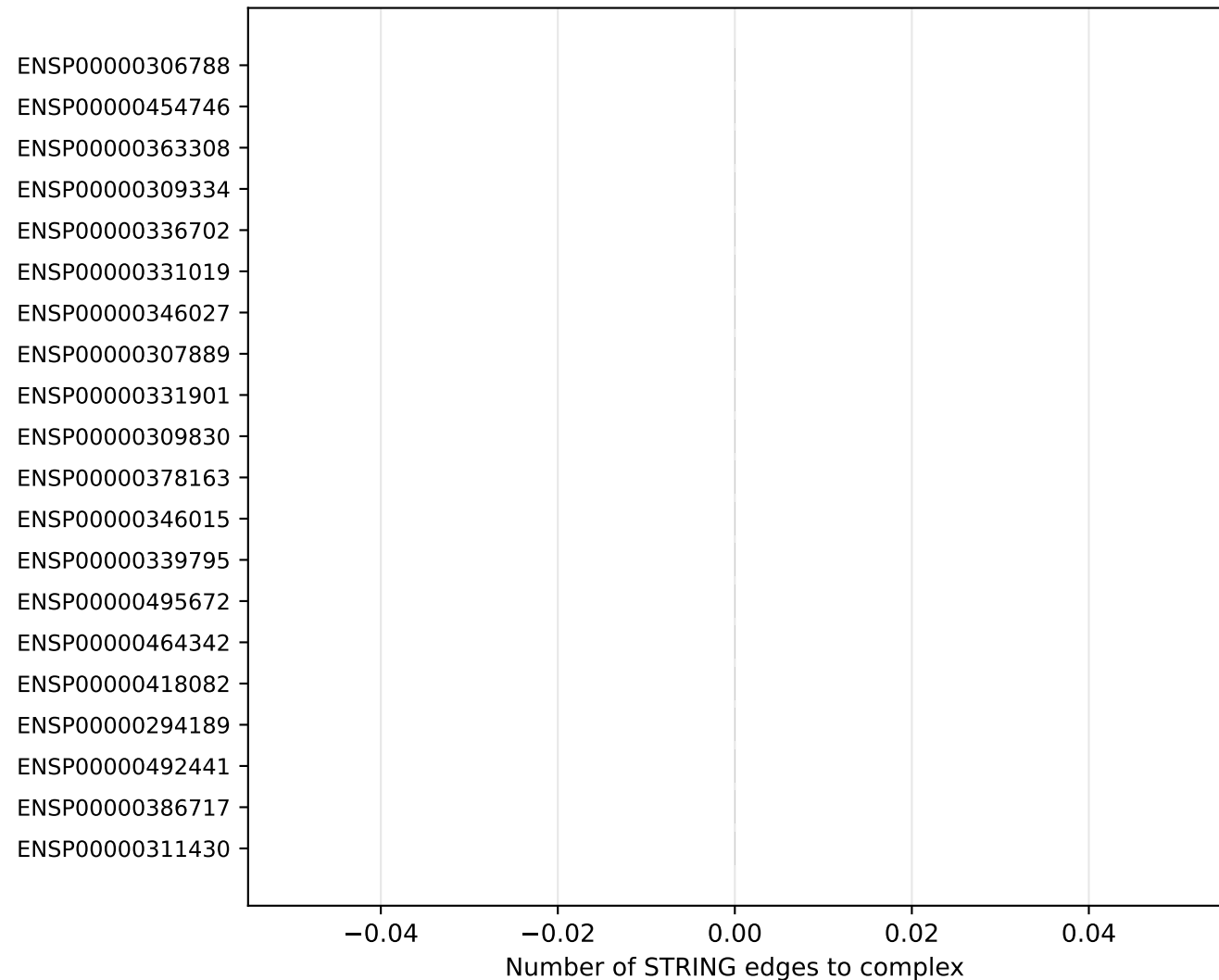
Ribosome, cytoplasmic: STRING evidence
