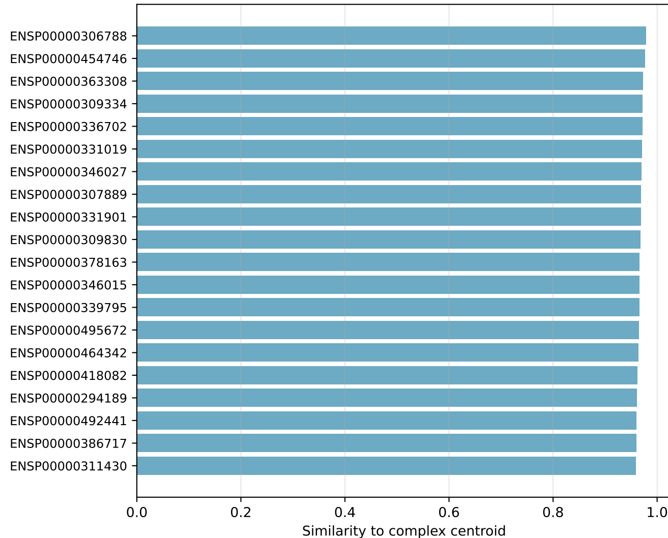
Ribosome, cytoplasmic: top candidates by embedding similarity
