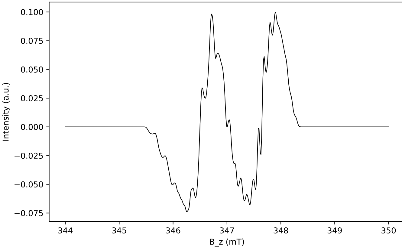
S7 — 5 nuclei (3 donor + 2 acceptor, max complexity)
