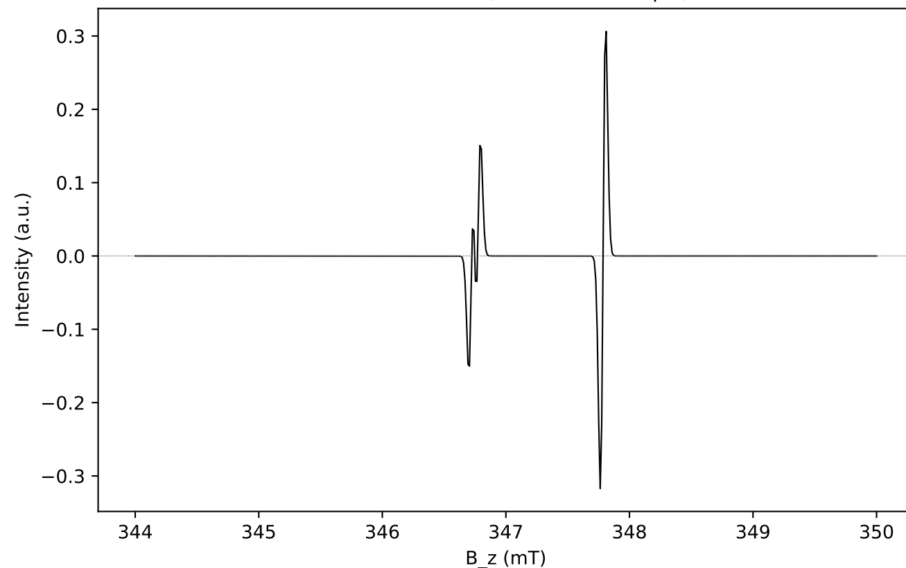
S4 — Swap of S3 (acceptor ^1\text{H} + donor 2\times^{14}\text{N} )
