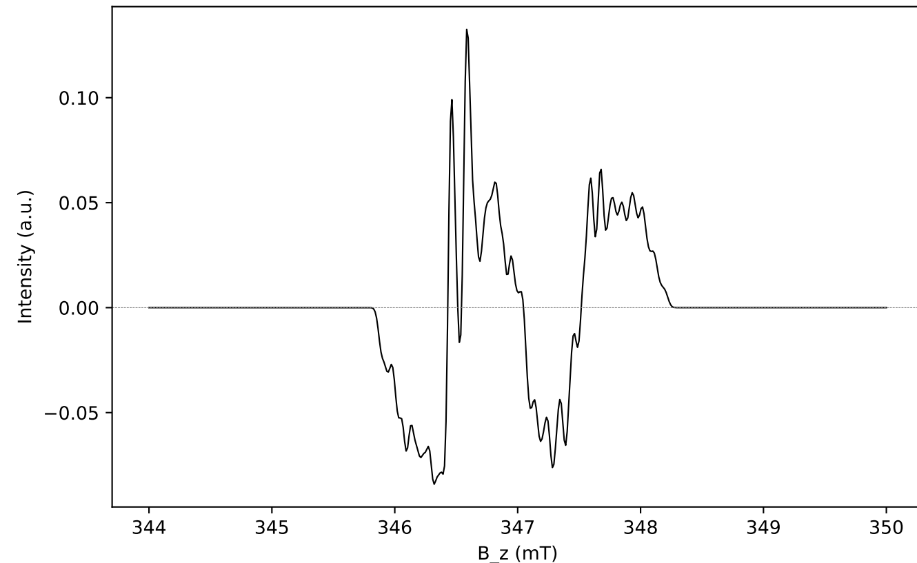
S5 — 3 nuclei (2 donor + 1 acceptor, n=3 methyl)
