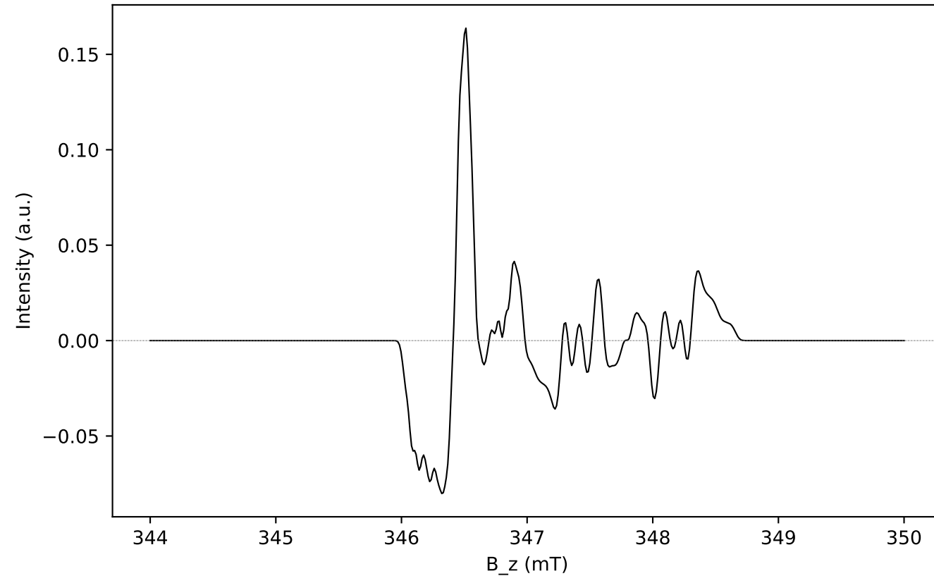
S6 — 4 nuclei (1 donor + 3 acceptor, I=3/2 ^{35}\text{Cl} )
