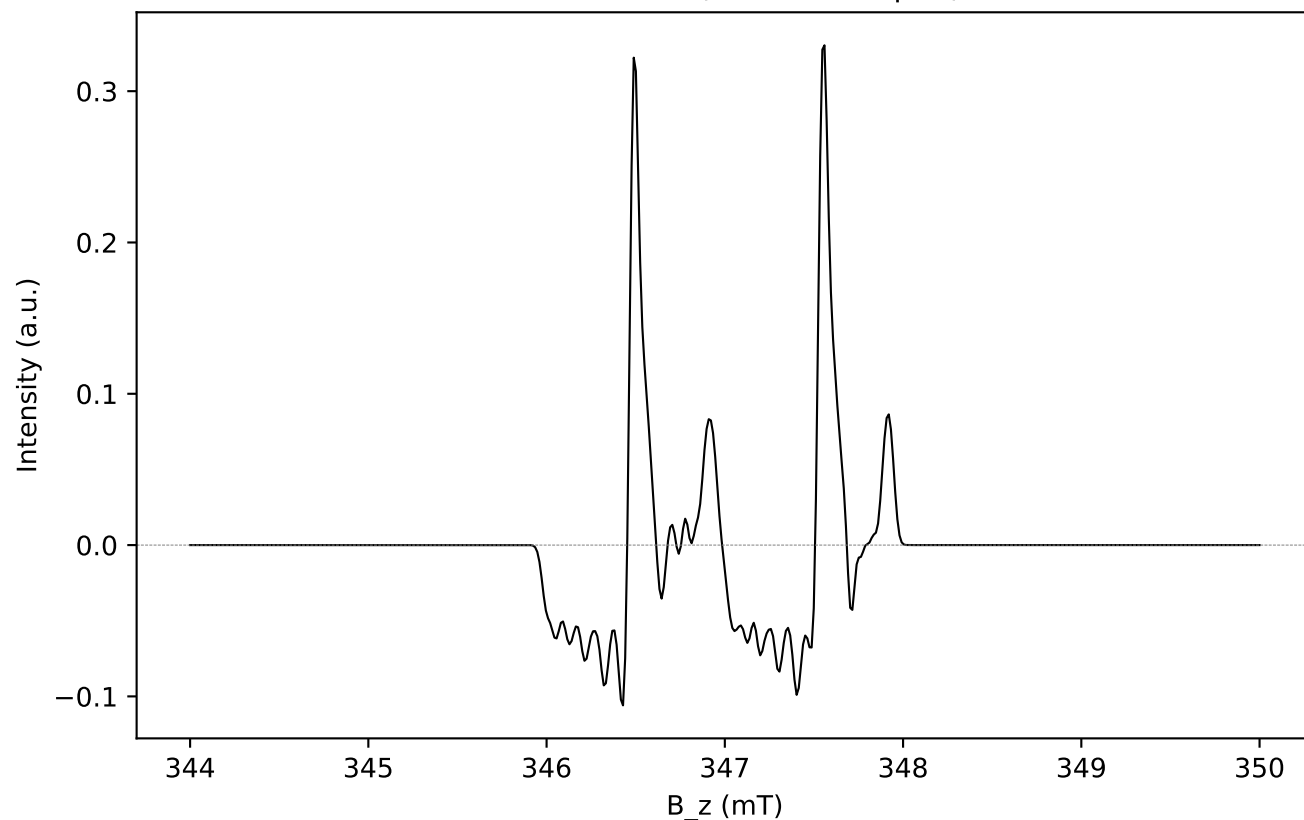
S3 — 2 nuclei (donor ^1\text{H} + acceptor 2\times^{14}\text{N} )
