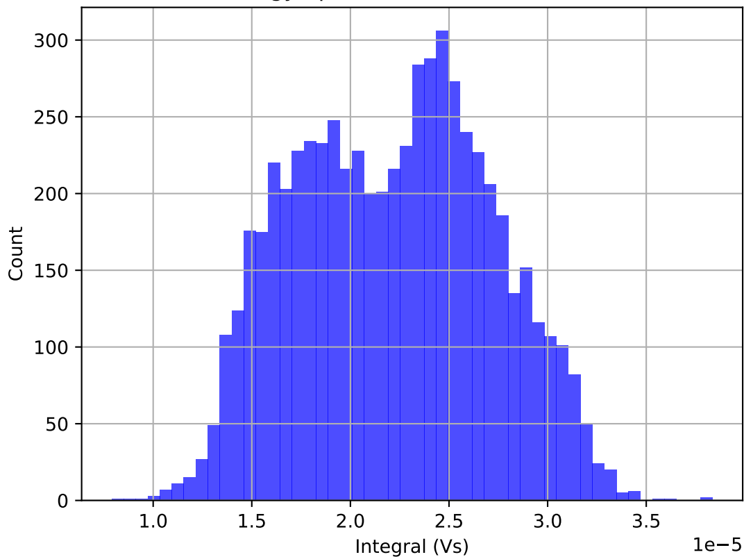
Energy Spectrum Ra226-270526-1
