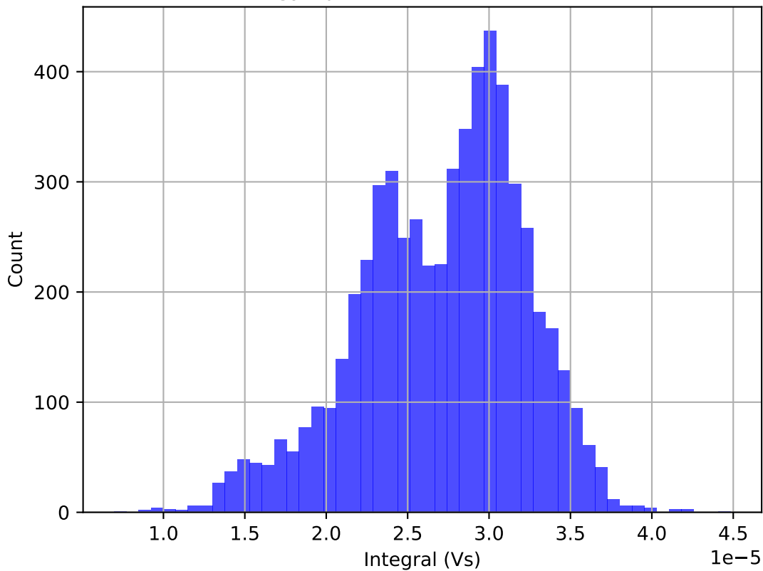
Energy Spectrum Ra226-270526-2
