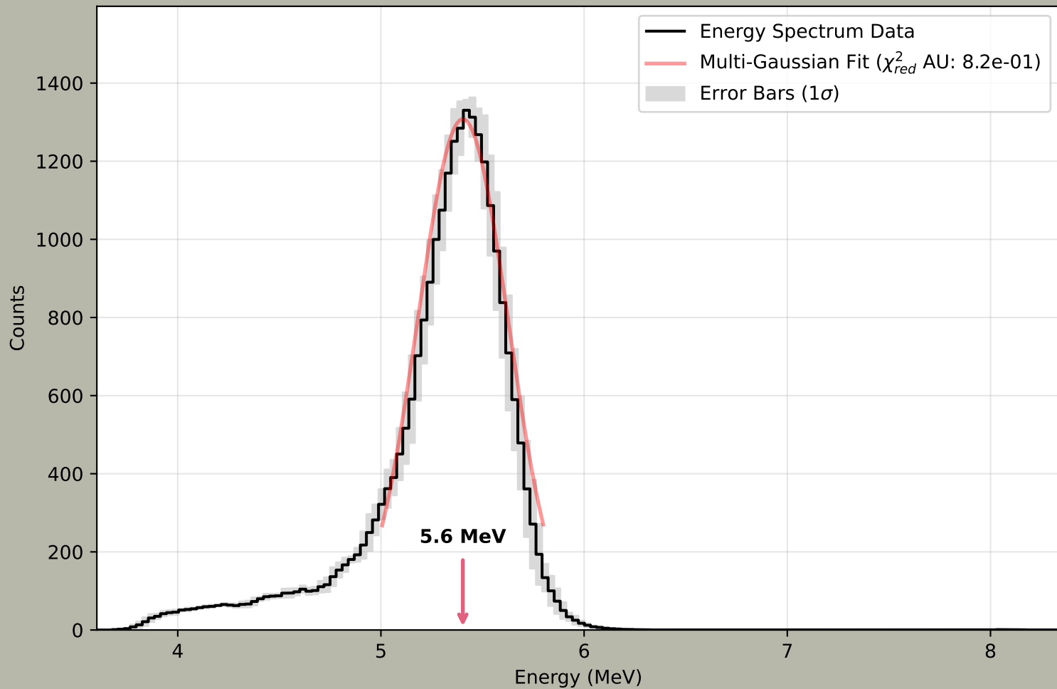
Calibrated Alpha Energy Spectrum - Am241
