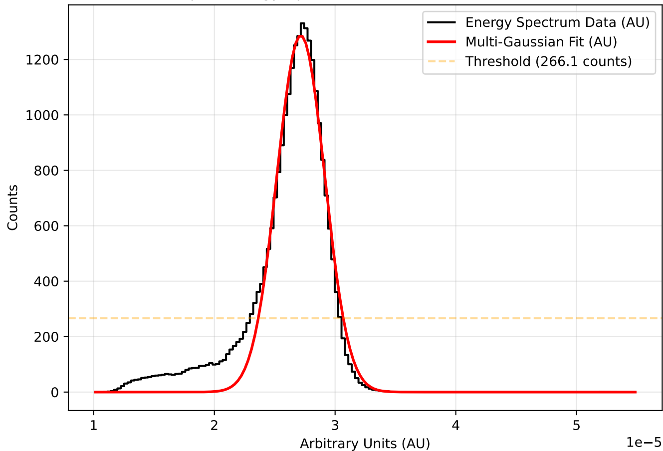
Alpha Energy Spectrum - Am241 (Uncalibrated)
