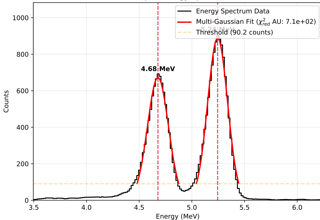
Calibrated Alpha Energy Spectrum - Pu239
