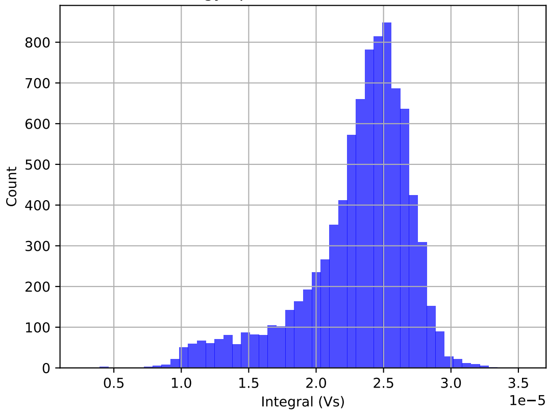
Energy Spectrum Am241-220526
