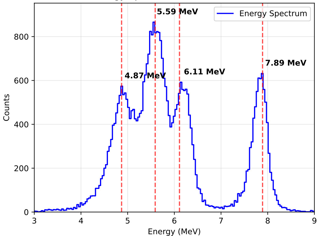
Energy Spectrum Ra226-290526-1
