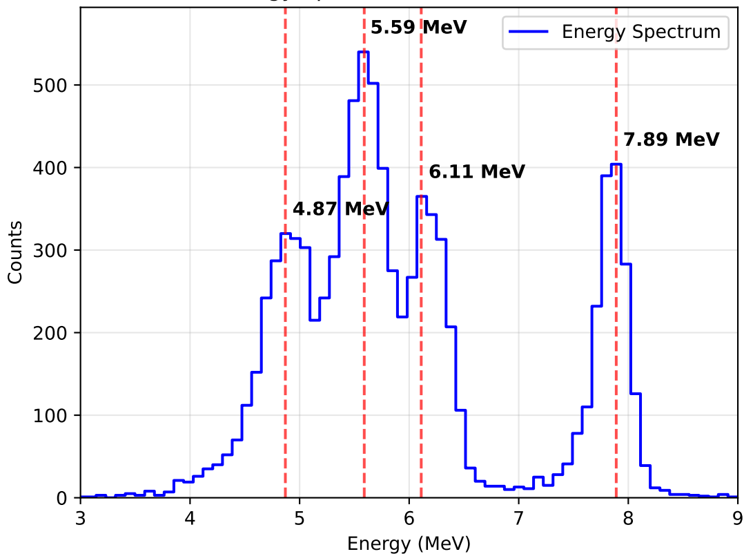
Energy Spectrum Ra226-290526-2
