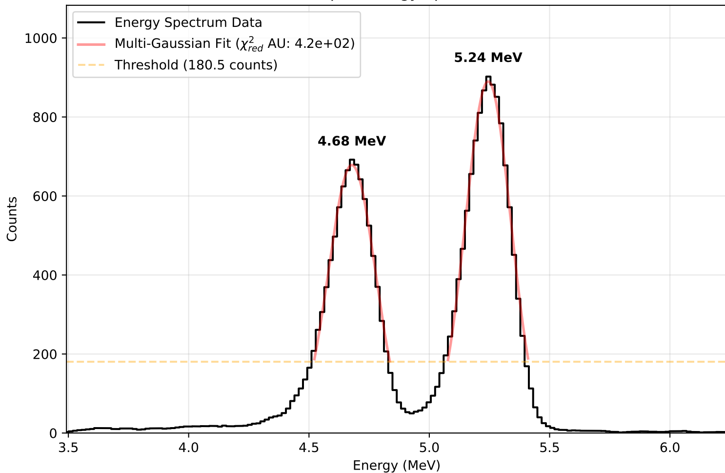
Calibrated Alpha Energy Spectrum - Pu239
