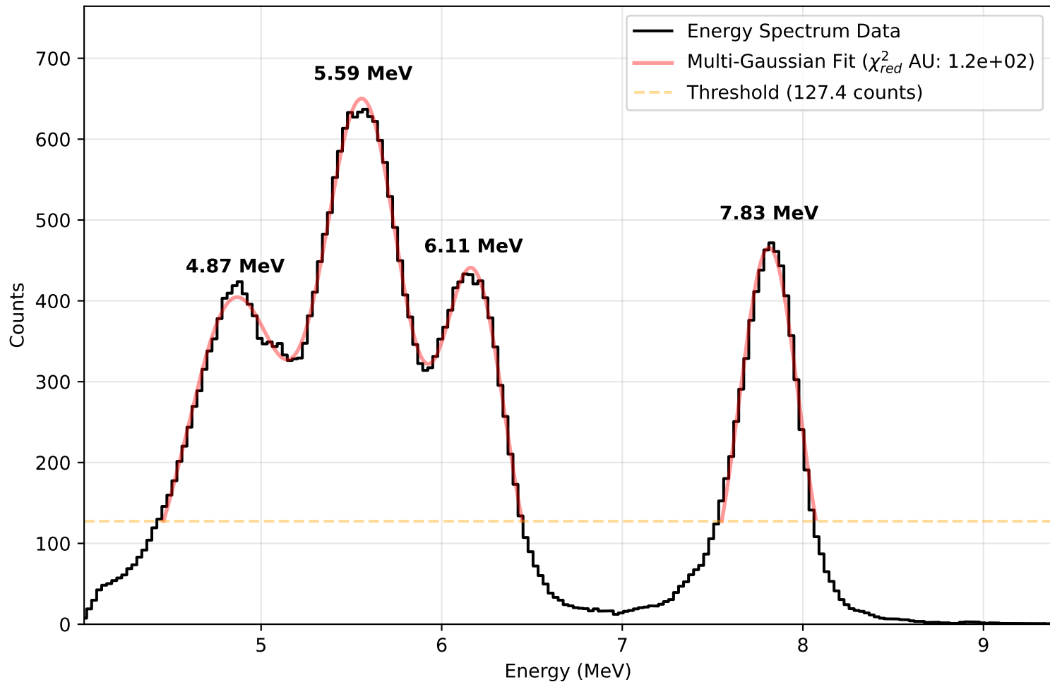
Calibrated Alpha Energy Spectrum - Ra226
