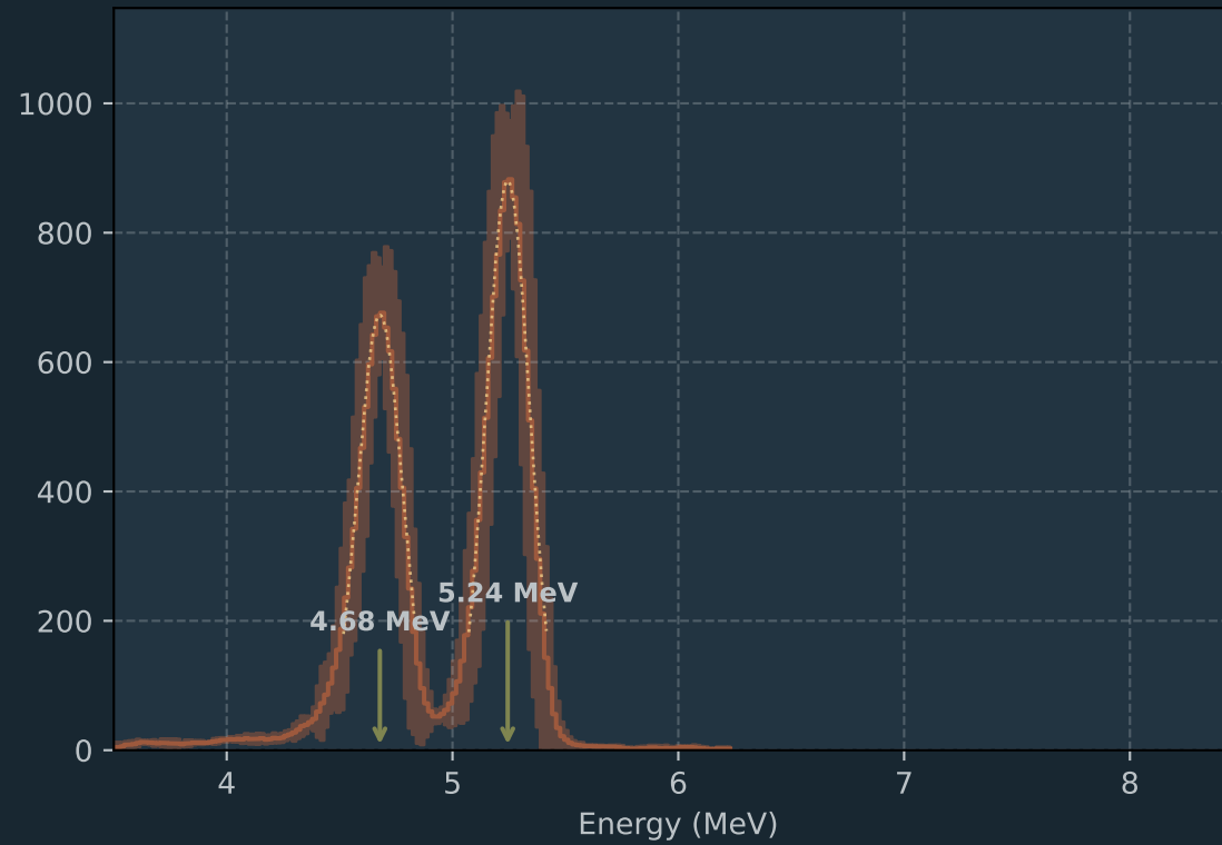
Pu239 Spectrum
