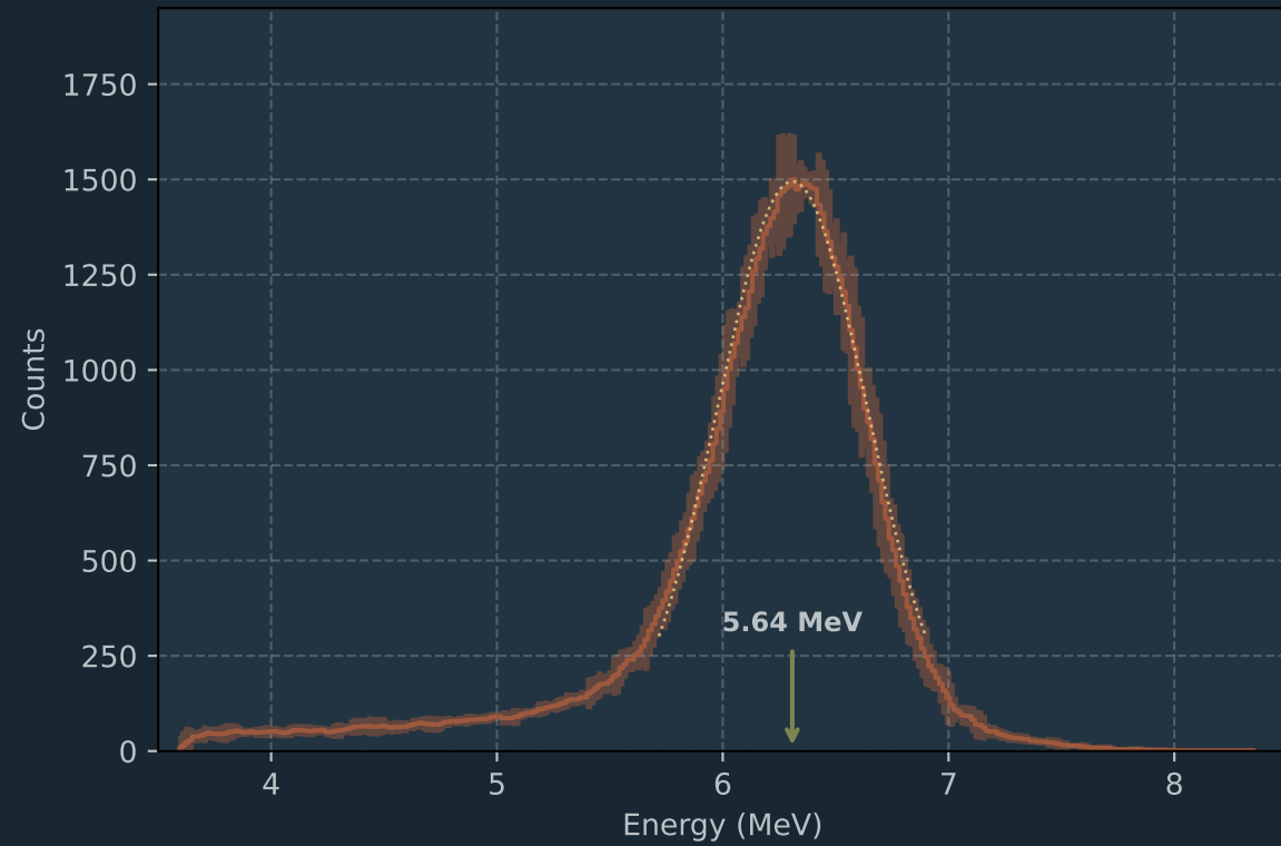
Am241 Spectrum
