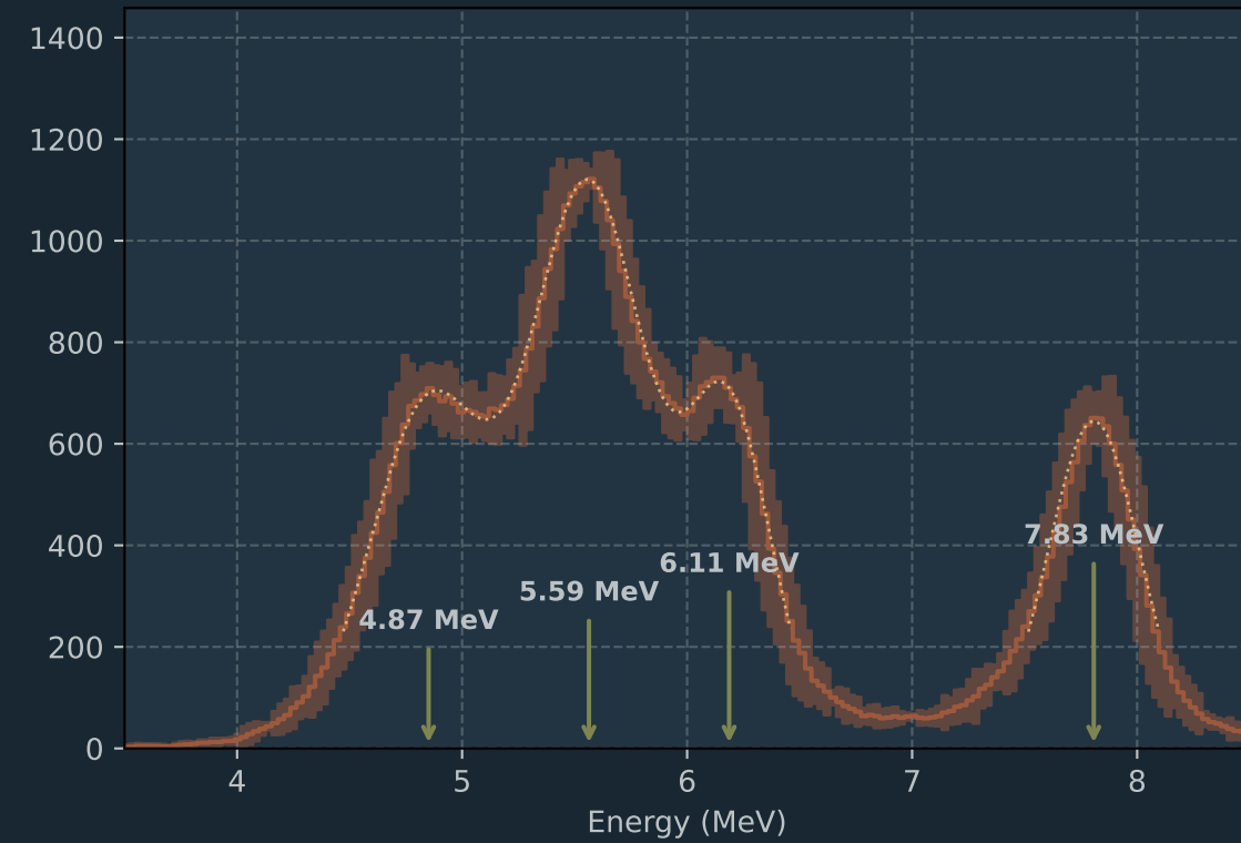
Ra226 Spectrum
