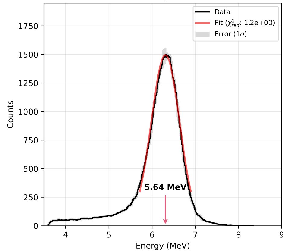
Am241 Spectrum
