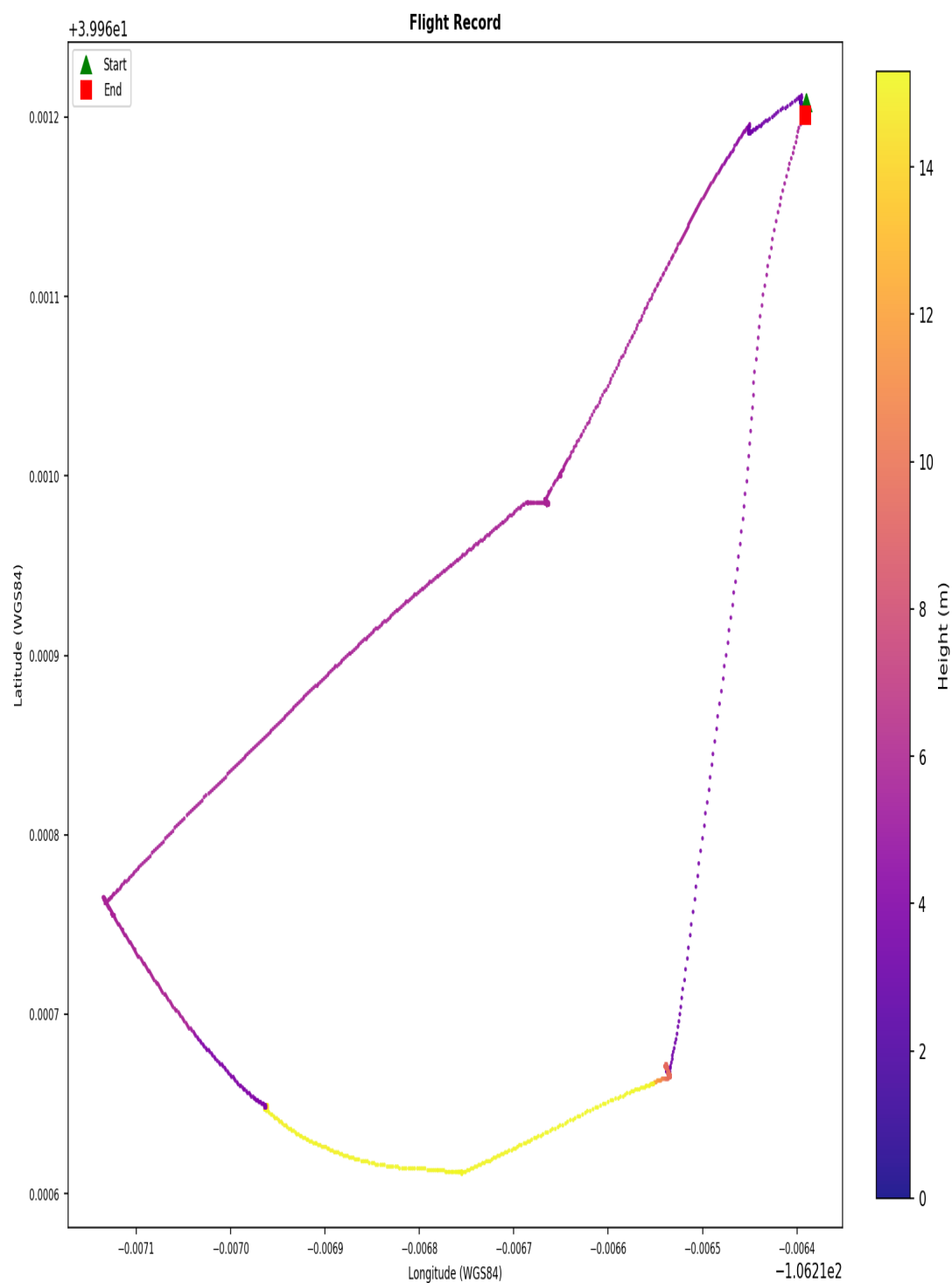
Flight Ground Track - flight_03
