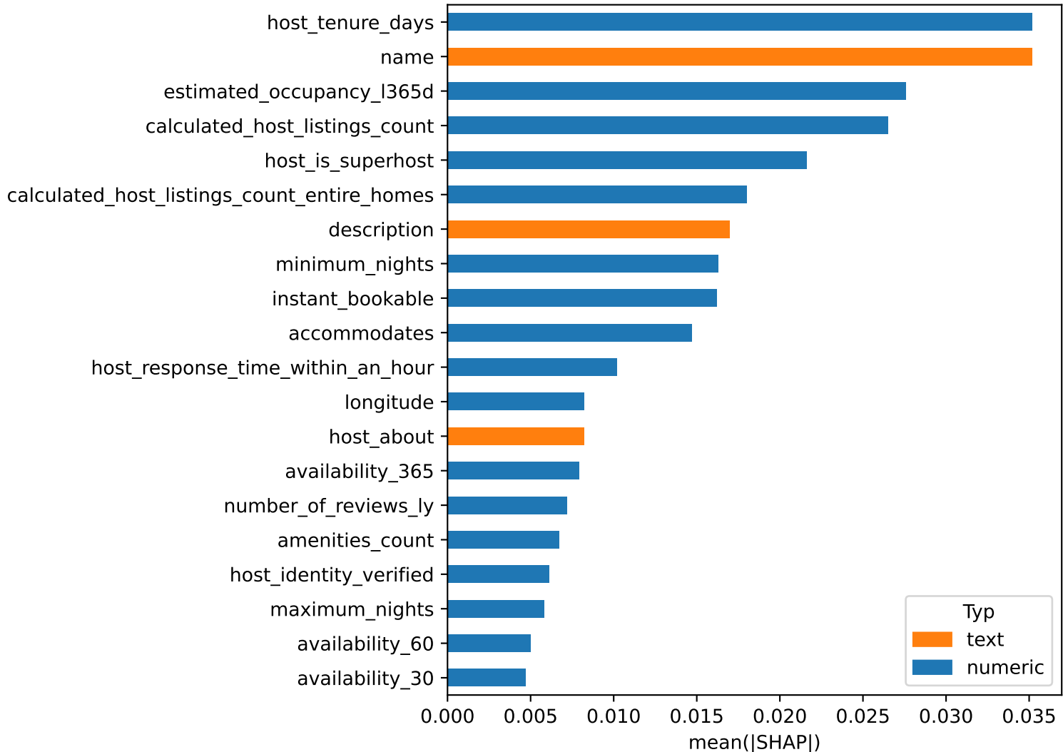
Exp 3 - airbnb_paris: Top 20 SHAP-Features
