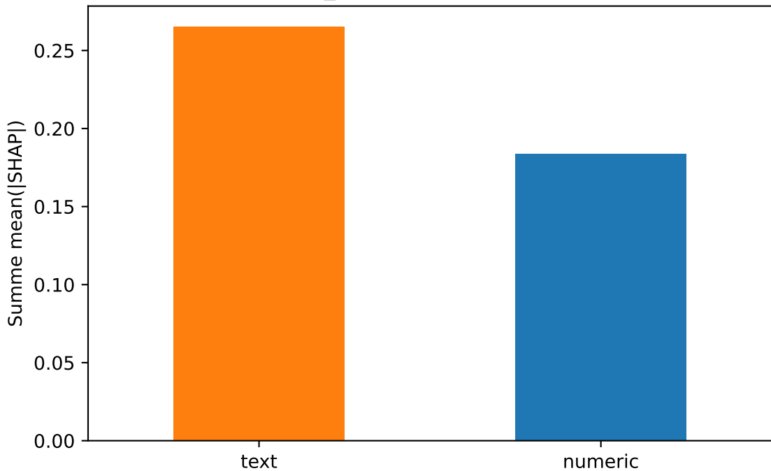
Exp 3 - fake_jobs: SHAP Text vs. numerisch
