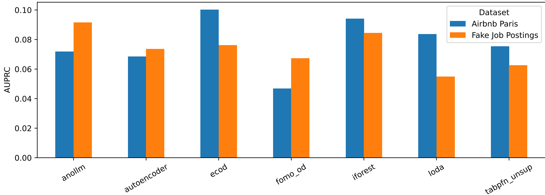
Experiment 1: AUPRC (both datasets)
