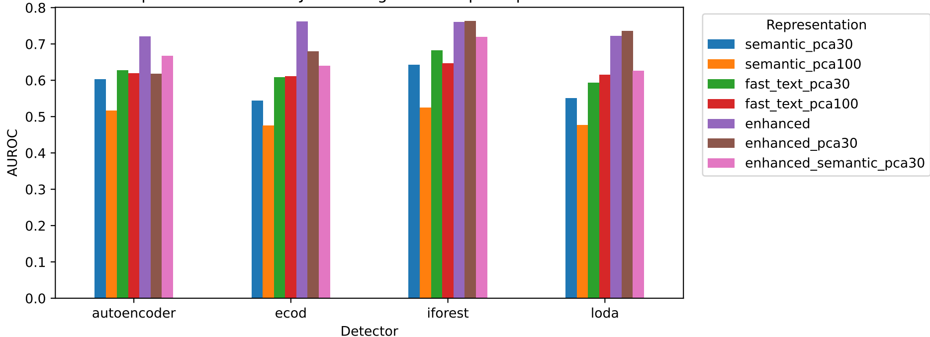
Experiment 2 on Fake Job Postings: AUROC per representation
