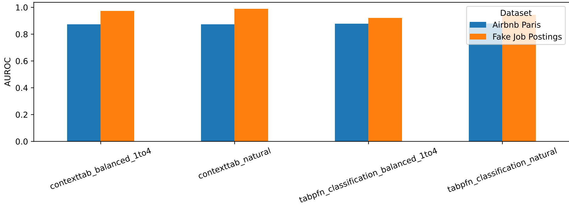
Experiment 3: AUROC (both datasets)
