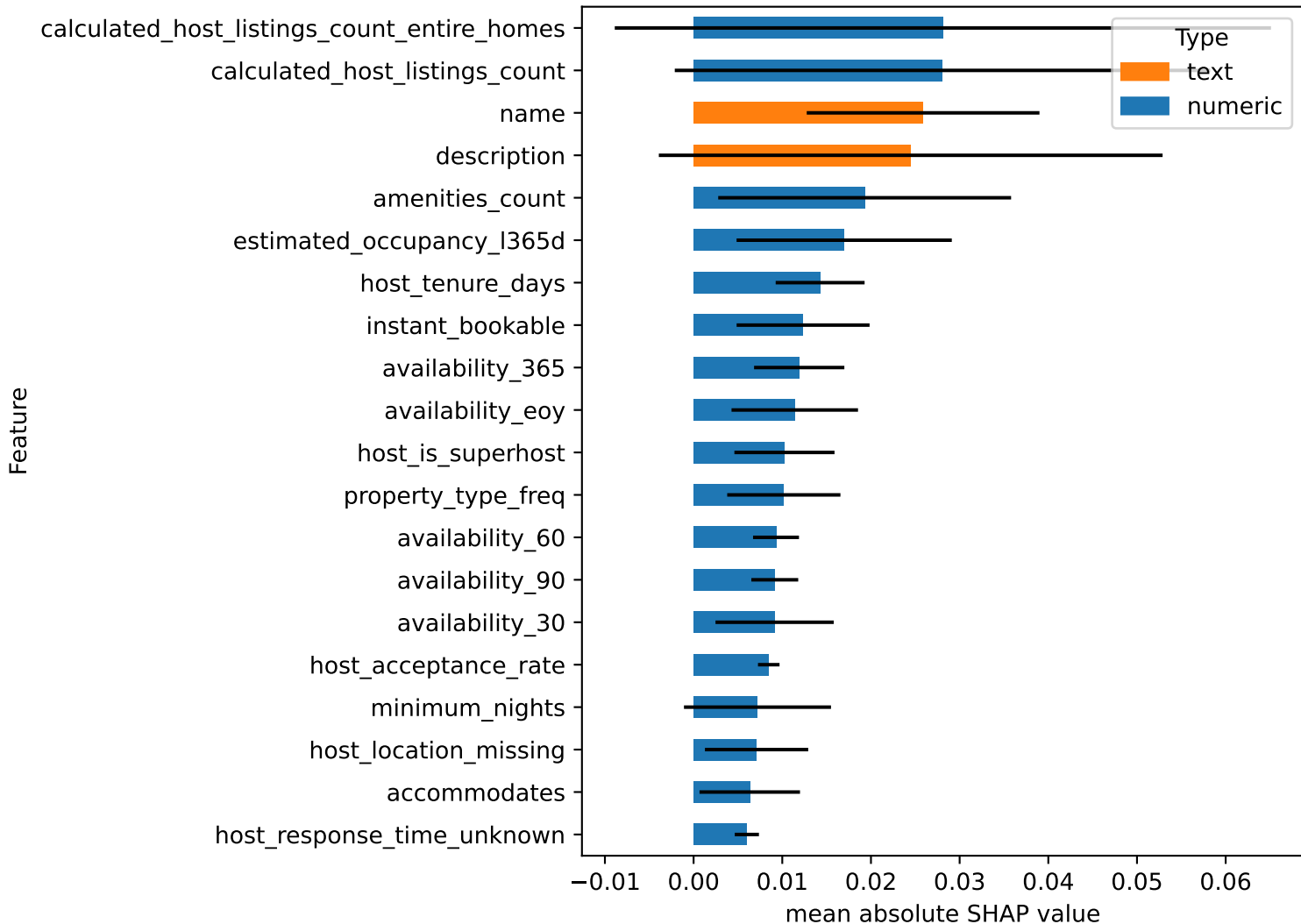
Preliminary experiment on Airbnb Paris: top 20 SHAP features
