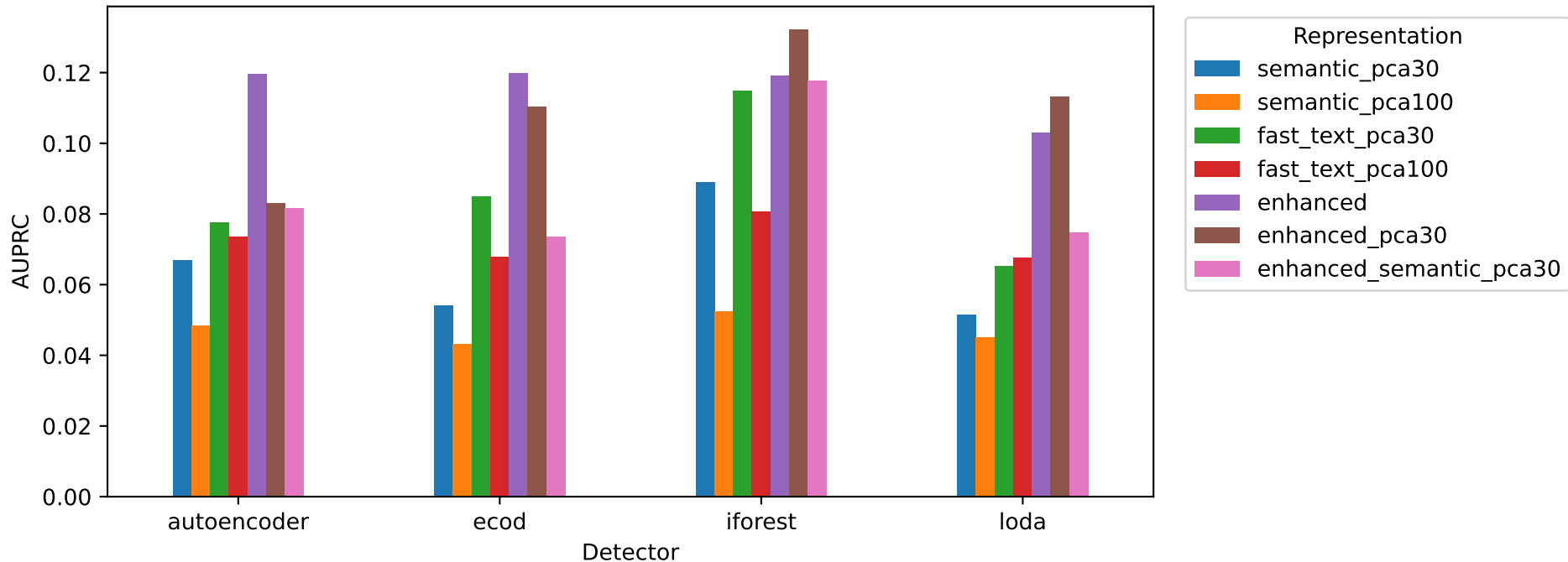
Experiment 2 on Fake Job Postings: AUPRC per representation
