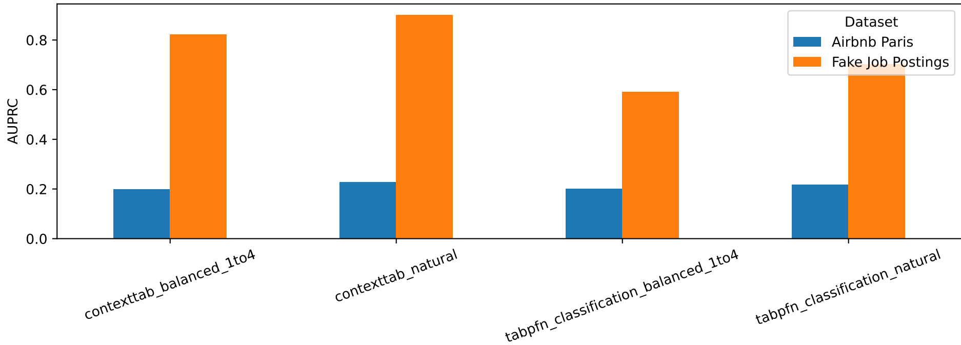
Experiment 3: AUPRC (both datasets)
